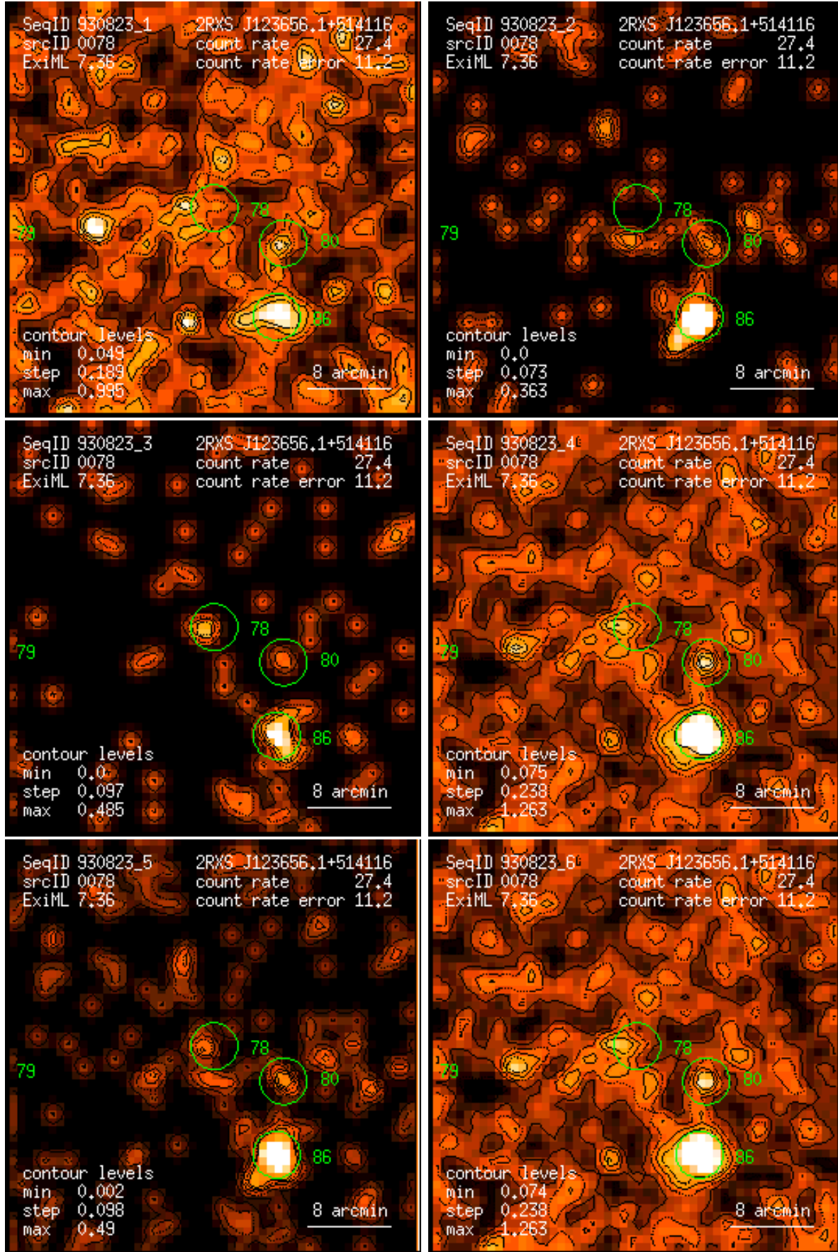
Figure 78: RASS 930823: detection 0078: band rate images, Gaussian filter: (1) PSPC channels 11 – 41, (2) 52 – 90, (3) 91 – 201, (4) 11 – 235, (5) 52 – 201, (6) 11 – 201. Broad band rates in counts/ks. Band rate contour levels in counts/ks/arcmin 2 .
