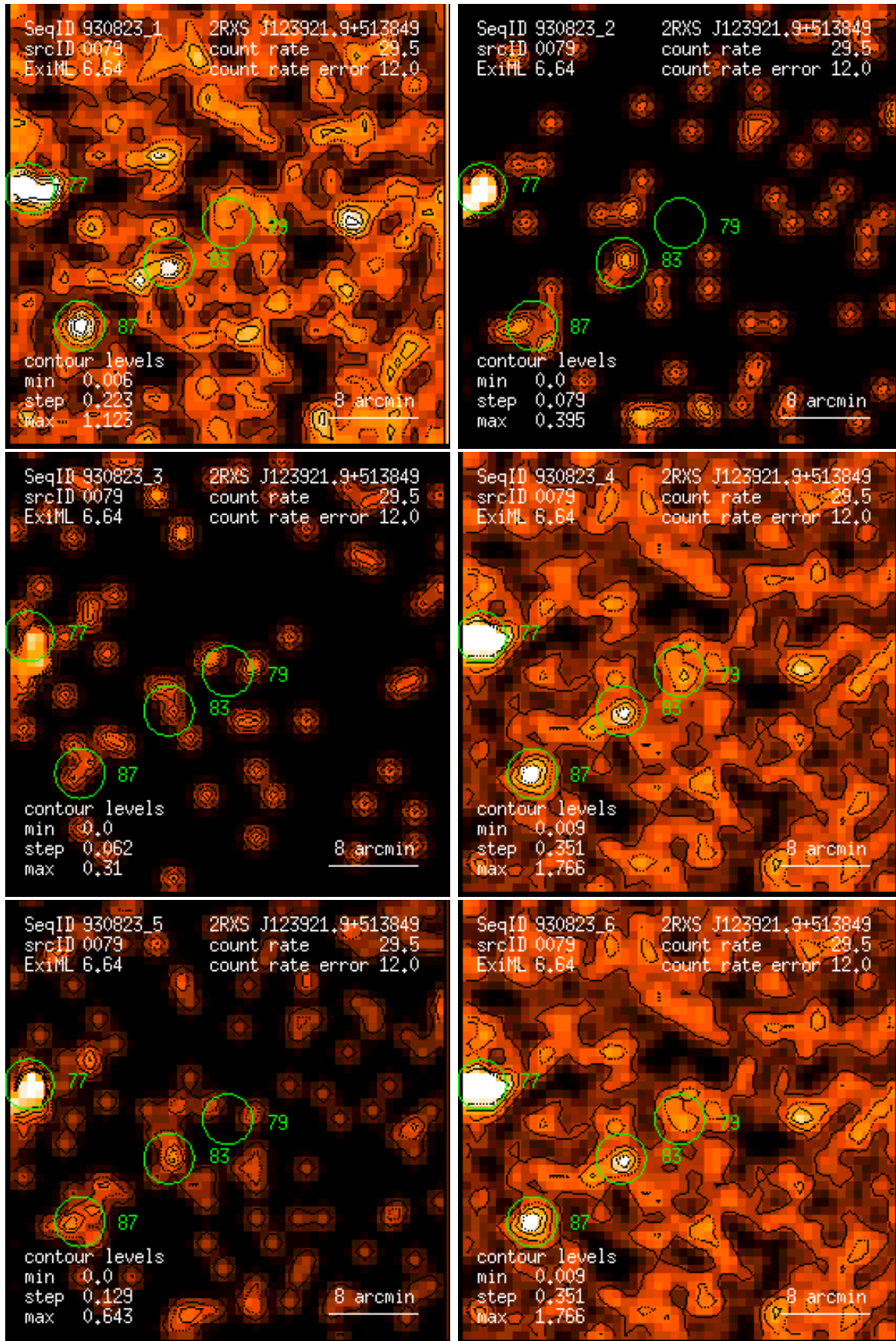
Figure 79: RASS 930823: detection 0079: band rate images, Gaussian filter: (1) PSPC channels 11 – 41, (2) 52 – 90, (3) 91 – 201, (4) 11 – 235, (5) 52 – 201, (6) 11 – 201. Broad band rates in counts/ks. Band rate contour levels in counts/ks/arcmin 2 .
