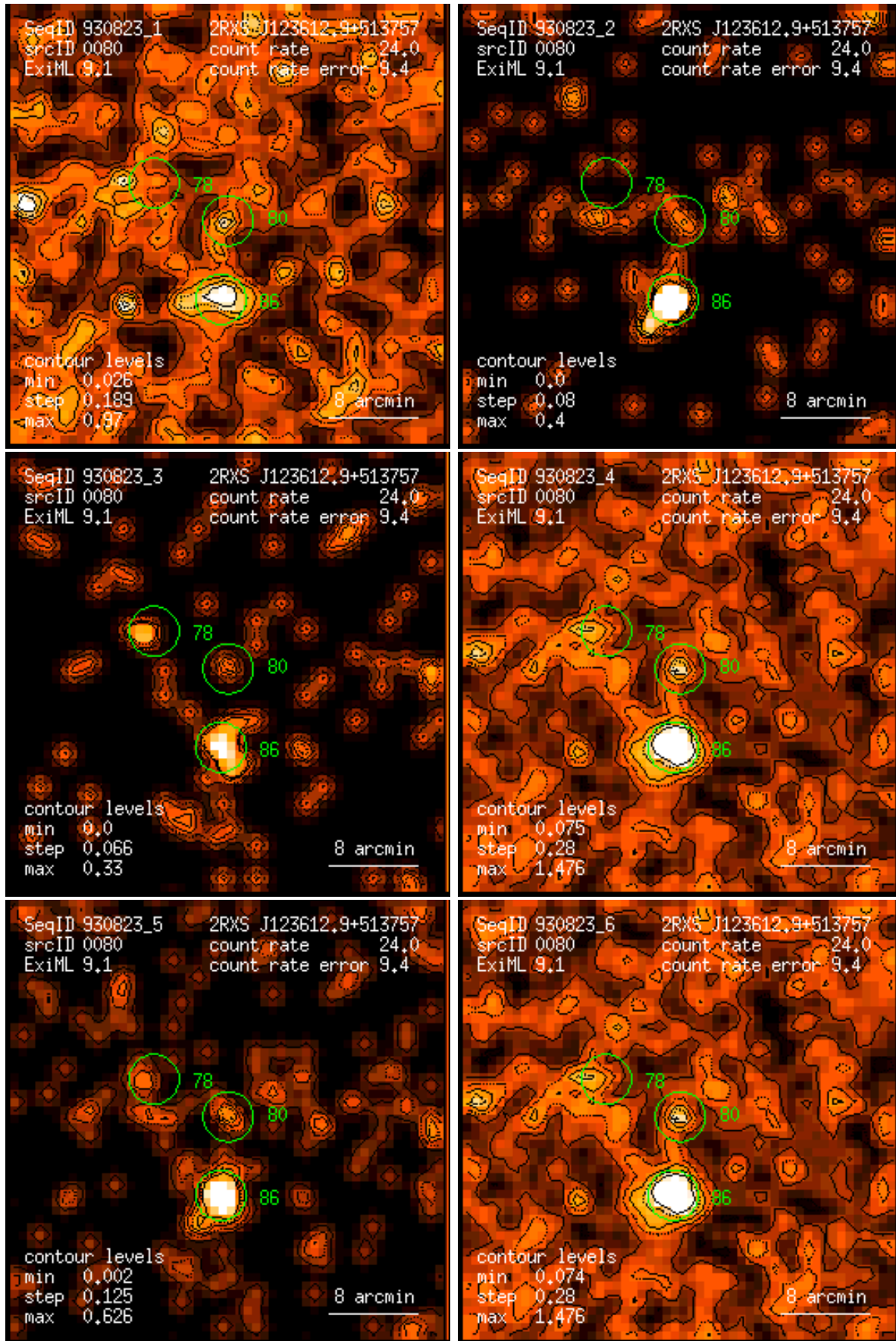
Figure 80: RASS 930823: detection 0080: band rate images, Gaussian filter: (1) PSPC channels 11 – 41, (2) 52 – 90, (3) 91 – 201, (4) 11 – 235, (5) 52 – 201, (6) 11 – 201. Broad band rates in counts/ks. Band rate contour levels in counts/ks/arcmin 2 .
