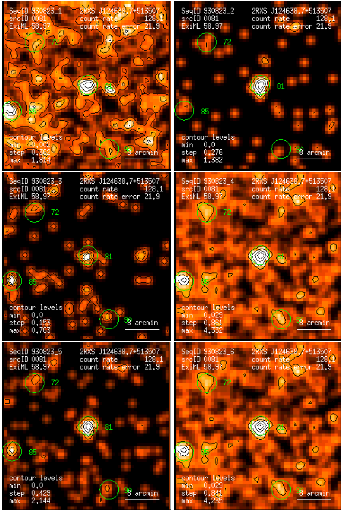
Figure 81: RASS 930823: detection 0081: band rate images, Gaussian filter: (1) PSPC channels 11 – 41, (2) 52 – 90, (3) 91 – 201, (4) 11 – 235, (5) 52 – 201, (6) 11 – 201. Broad band rates in counts/ks. Band rate contour levels in counts/ks/arcmin 2 .
