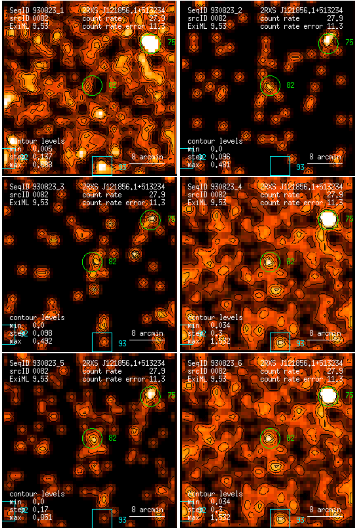
Figure 82: RASS 930823: detection 0082: band rate images, Gaussian filter: (1) PSPC channels 11 – 41, (2) 52 – 90, (3) 91 – 201, (4) 11 – 235, (5) 52 – 201, (6) 11 – 201. Broad band rates in counts/ks. Band rate contour levels in counts/ks/arcmin 2 .
