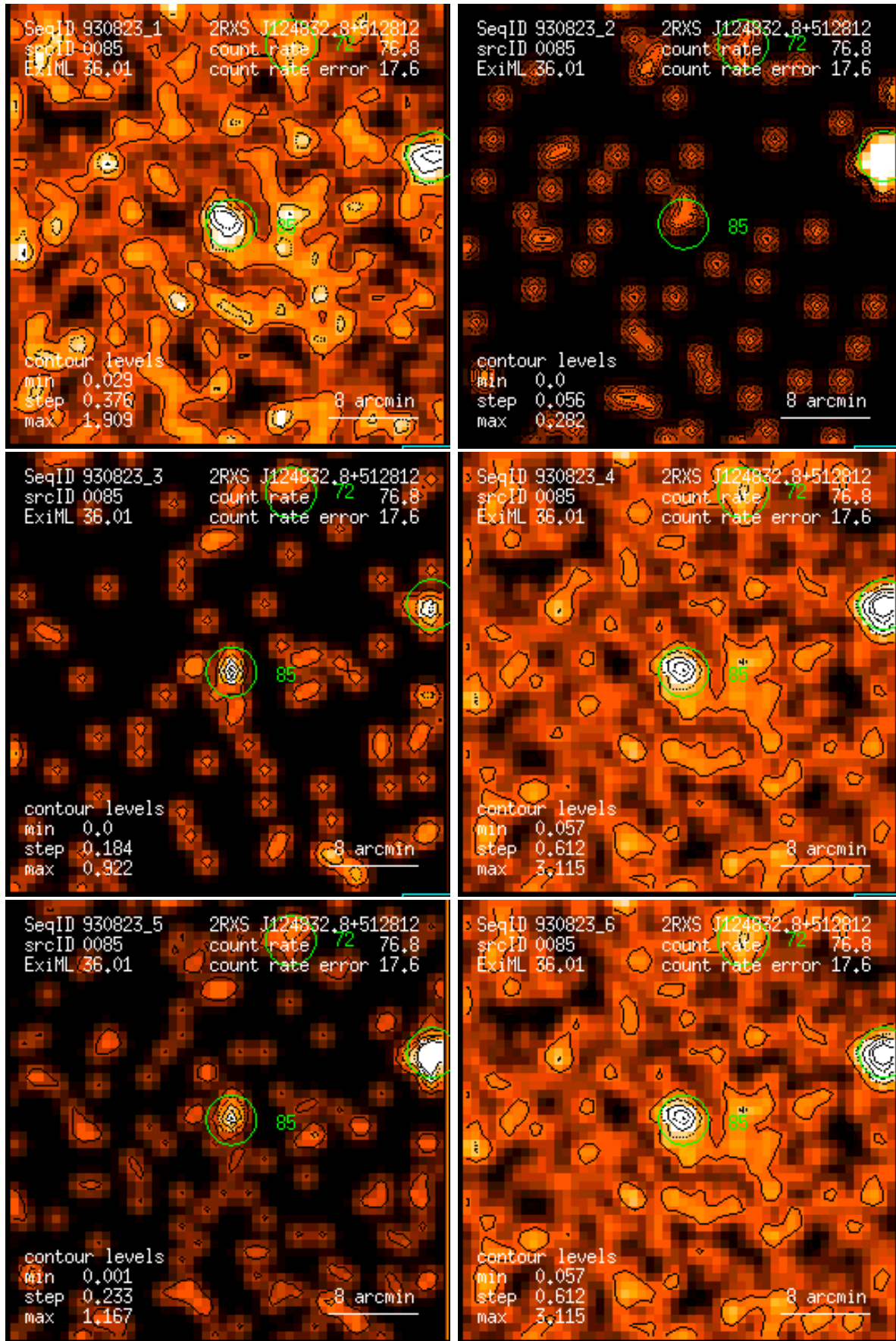
Figure 85: RASS 930823: detection 0085: band rate images, Gaussian filter: (1) PSPC channels 11 – 41, (2) 52 – 90, (3) 91 – 201, (4) 11 – 235, (5) 52 – 201, (6) 11 – 201. Broad band rates in counts/ks. Band rate contour levels in counts/ks/arcmin 2 .
