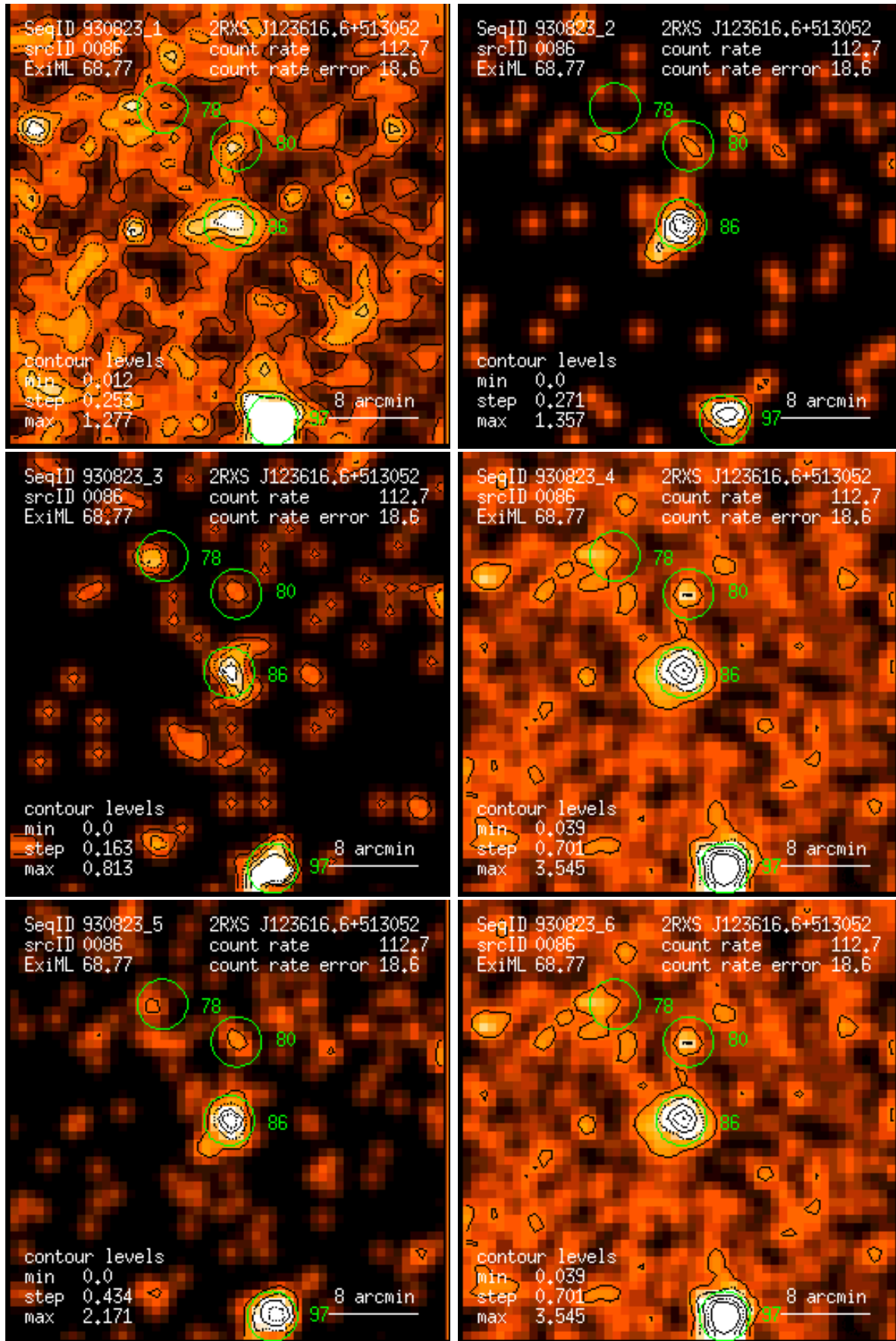
Figure 86: RASS 930823: detection 0086: band rate images, Gaussian filter: (1) PSPC channels 11 – 41, (2) 52 – 90, (3) 91 – 201, (4) 11 – 235, (5) 52 – 201, (6) 11 – 201. Broad band rates in counts/ks. Band rate contour levels in counts/ks/arcmin 2 .
