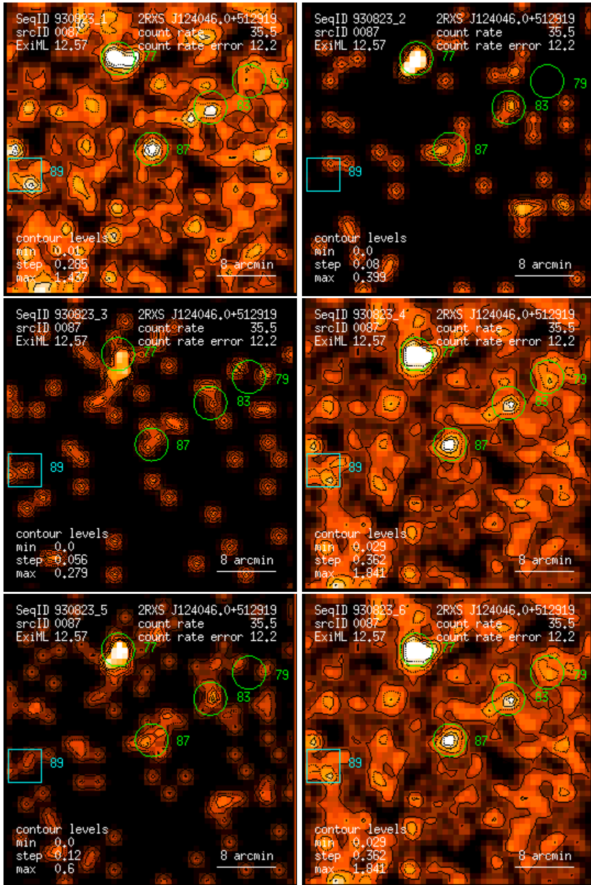
Figure 87: RASS 930823: detection 0087: band rate images, Gaussian filter: (1) PSPC channels 11 – 41, (2) 52 – 90, (3) 91 – 201, (4) 11 – 235, (5) 52 – 201, (6) 11 – 201. Broad band rates in counts/ks. Band rate contour levels in counts/ks/arcmin 2 .
