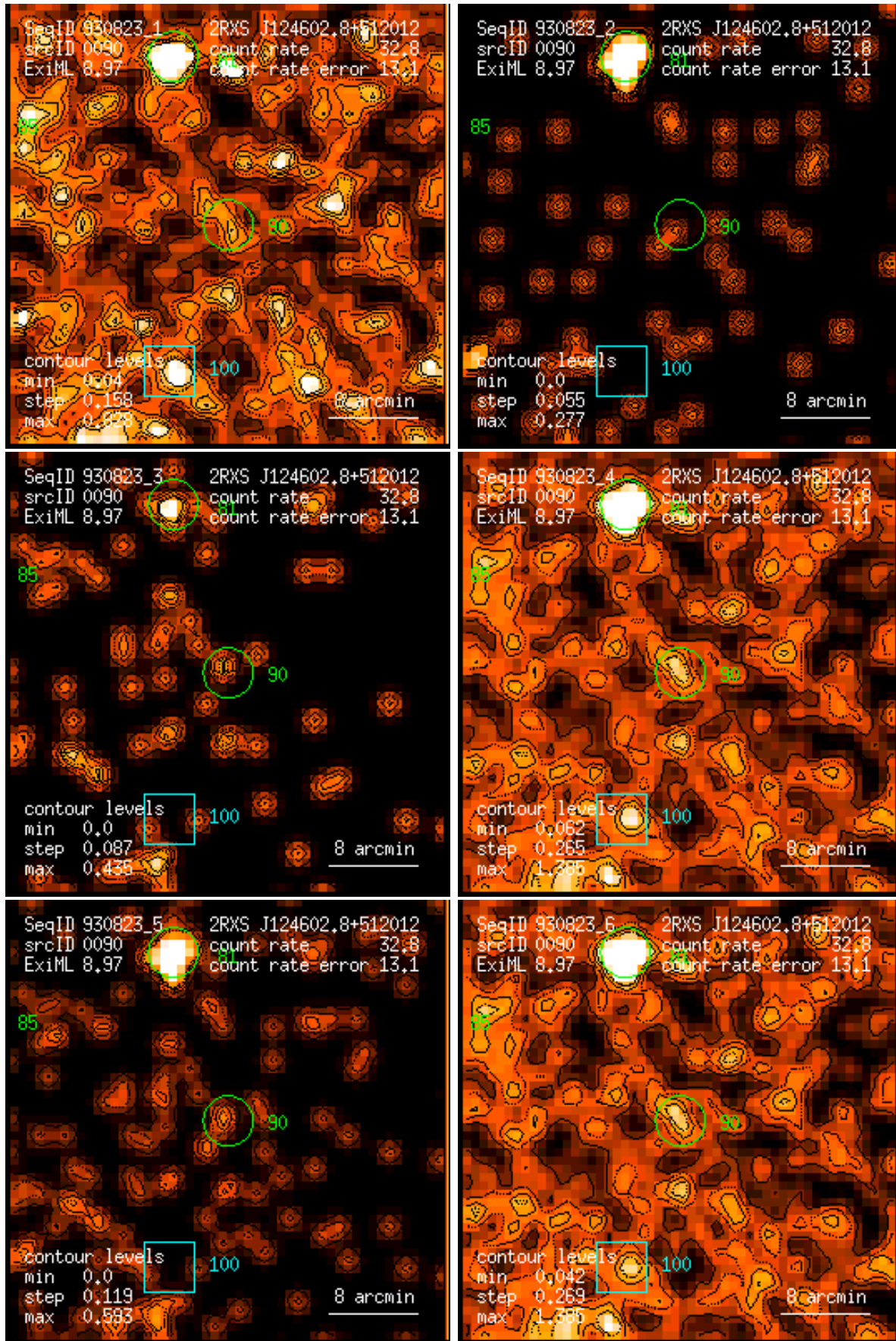
Figure 90: RASS 930823: detection 0090: band rate images, Gaussian filter: (1) PSPC channels 11 – 41, (2) 52 – 90, (3) 91 – 201, (4) 11 – 235, (5) 52 – 201, (6) 11 – 201. Broad band rates in counts/ks. Band rate contour levels in counts/ks/arcmin 2 .
