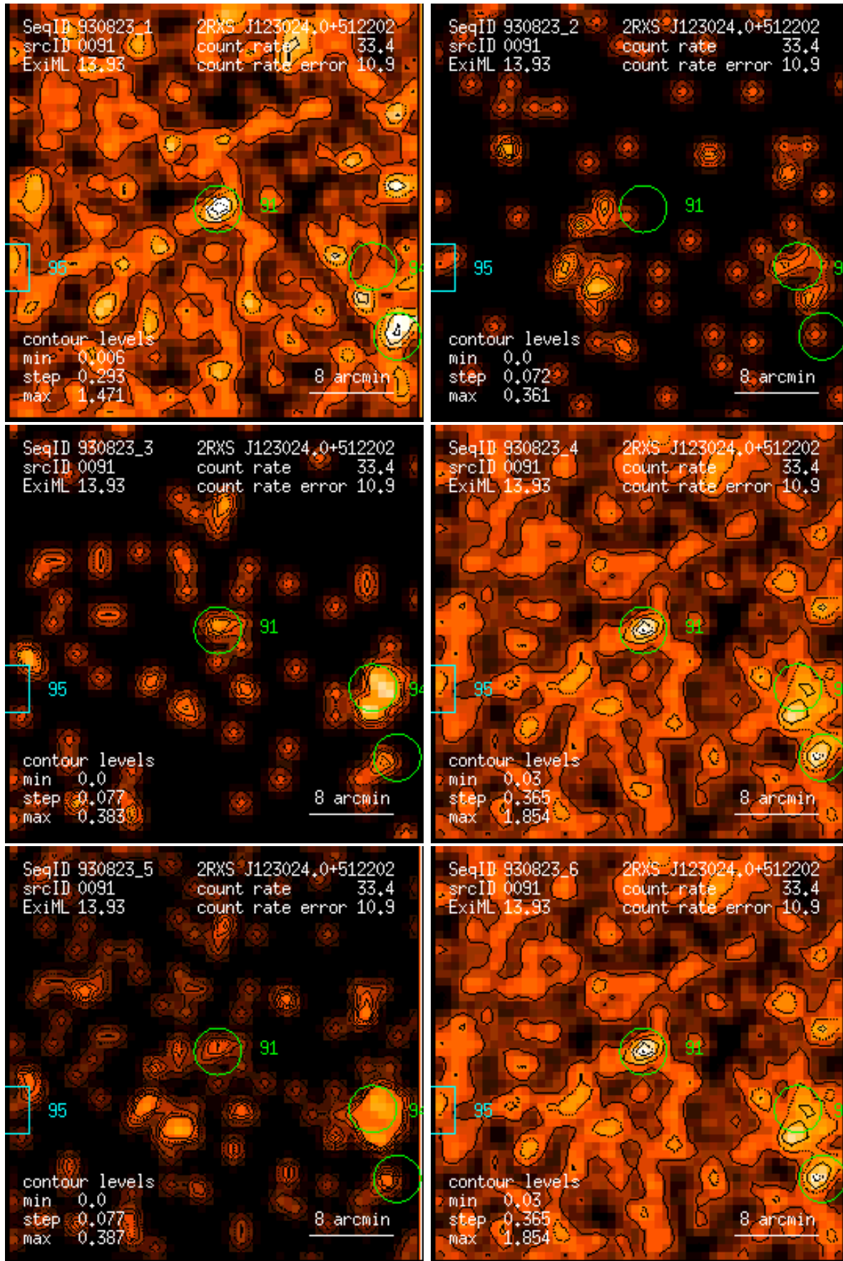
Figure 91: RASS 930823: detection 0091: band rate images, Gaussian filter: (1) PSPC channels 11 – 41, (2) 52 – 90, (3) 91 – 201, (4) 11 – 235, (5) 52 – 201, (6) 11 – 201. Broad band rates in counts/ks. Band rate contour levels in counts/ks/arcmin 2 .
