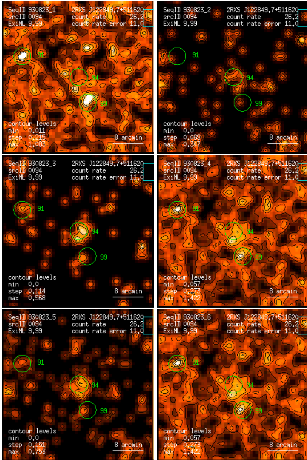
Figure 94: RASS 930823: detection 0094: band rate images, Gaussian filter: (1) PSPC channels 11 – 41, (2) 52 – 90, (3) 91 – 201, (4) 11 – 235, (5) 52 – 201, (6) 11 – 201. Broad band rates in counts/ks. Band rate contour levels in counts/ks/arcmin 2 .
