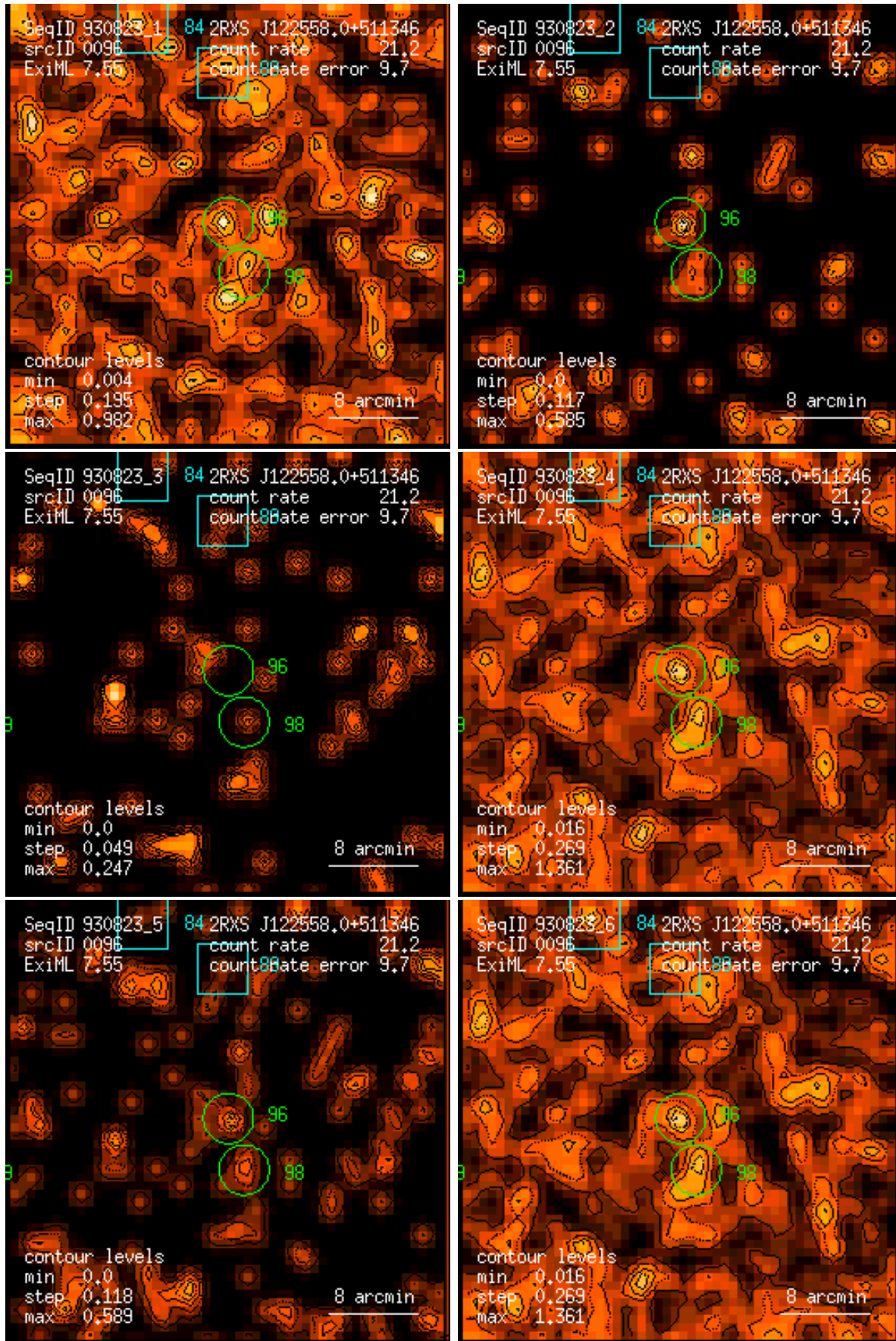
Figure 96: RASS 930823: detection 0096: band rate images, Gaussian filter: (1) PSPC channels 11 – 41, (2) 52 – 90, (3) 91 – 201, (4) 11 – 235, (5) 52 – 201, (6) 11 – 201. Broad band rates in counts/ks. Band rate contour levels in counts/ks/arcmin 2 .
