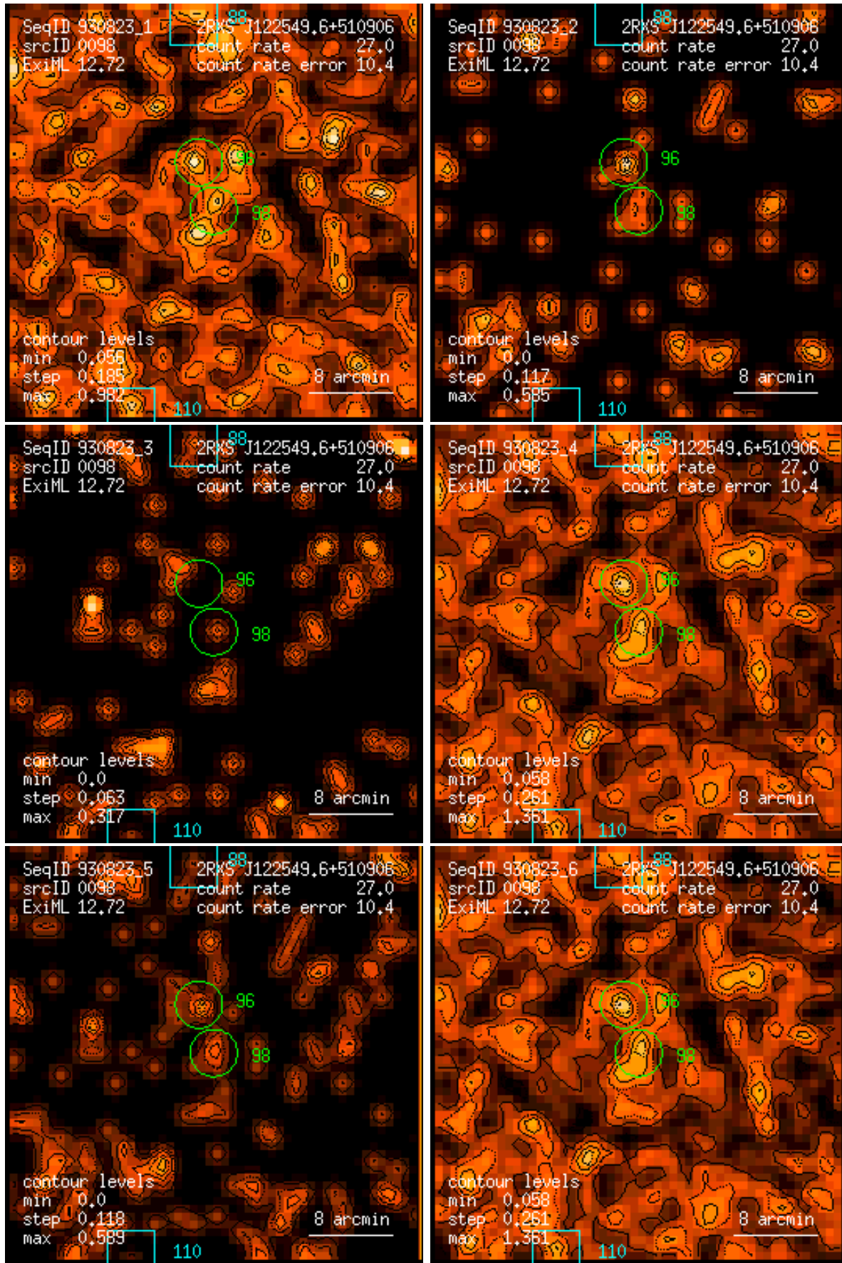
Figure 98: RASS 930823: detection 0098: band rate images, Gaussian filter: (1) PSPC channels 11 – 41, (2) 52 – 90, (3) 91 – 201, (4) 11 – 235, (5) 52 – 201, (6) 11 – 201. Broad band rates in counts/ks. Band rate contour levels in counts/ks/arcmin 2 .
