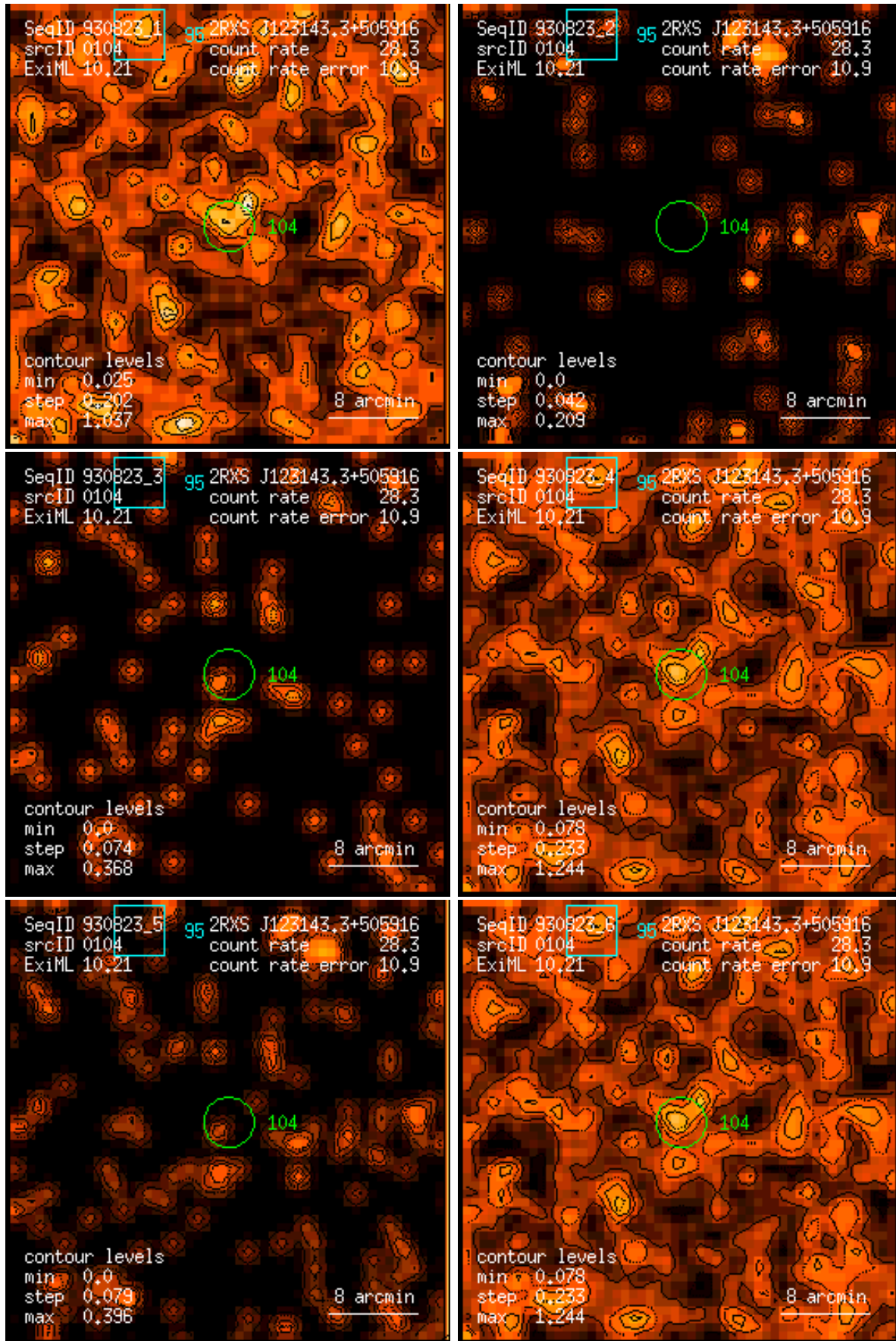
Figure 104: RASS 930823: detection 0104: band rate images, Gaussian filter: (1) PSPC channels 11 – 41, (2) 52 – 90, (3) 91 – 201, (4) 11 – 235, (5) 52 – 201, (6) 11 – 201. Broad band rates in counts/ks. Band rate contour levels in counts/ks/arcmin 2 .
