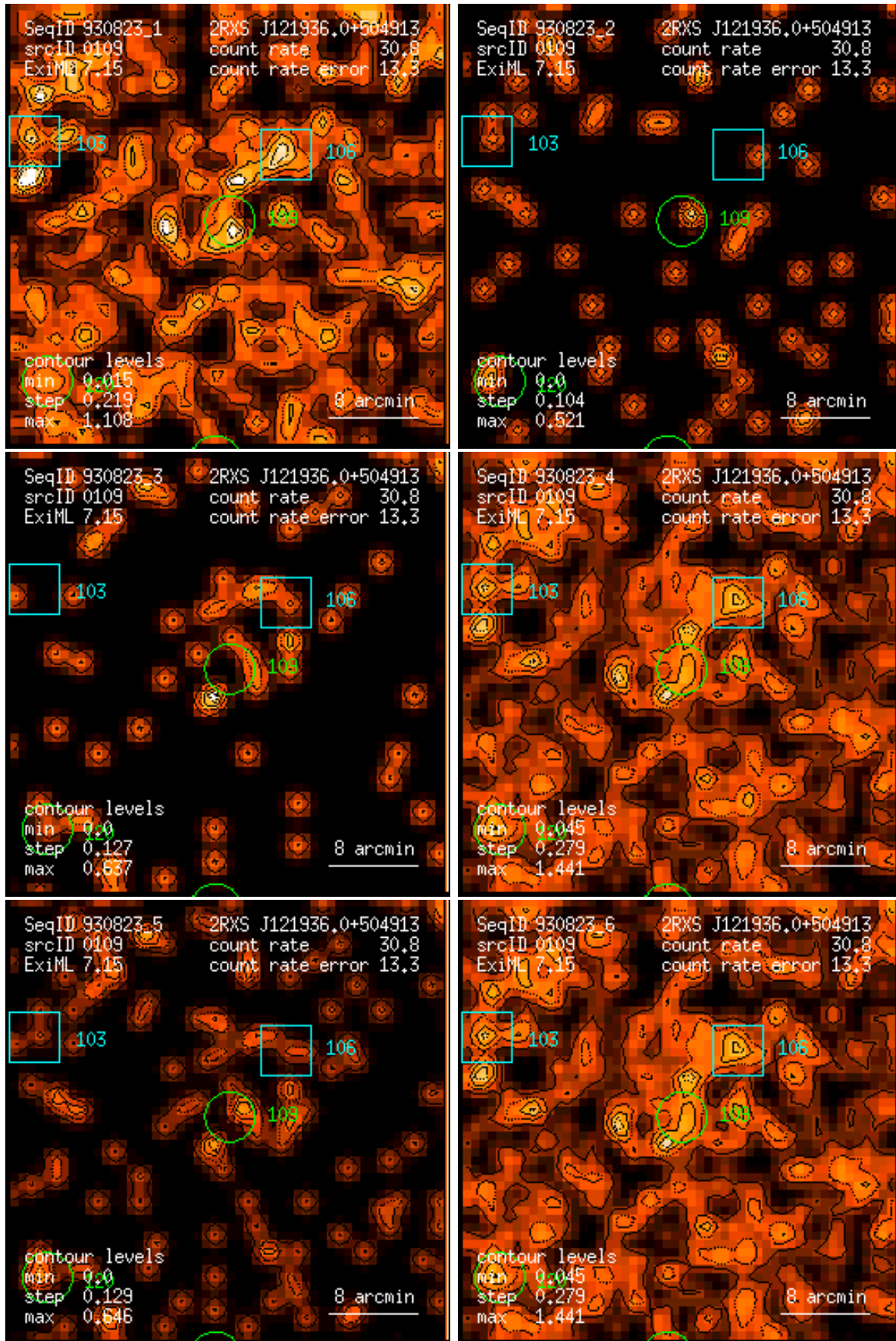
Figure 109: RASS 930823: detection 0109: band rate images, Gaussian filter: (1) PSPC channels 11 – 41, (2) 52 – 90, (3) 91 – 201, (4) 11 – 235, (5) 52 – 201, (6) 11 – 201. Broad band rates in counts/ks. Band rate contour levels in counts/ks/arcmin 2 .
