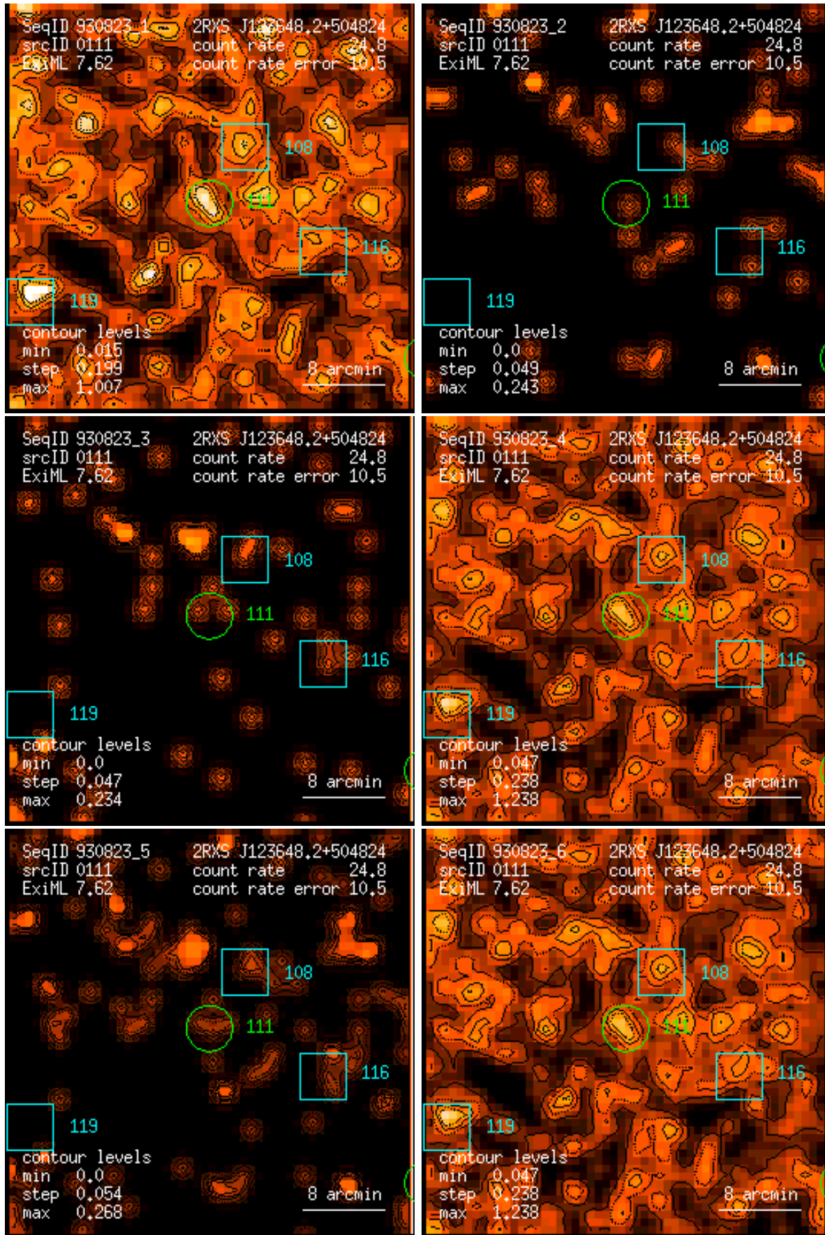
Figure 111: RASS 930823: detection 0111: band rate images, Gaussian filter: (1) PSPC channels 11 – 41, (2) 52 – 90, (3) 91 – 201, (4) 11 – 235, (5) 52 – 201, (6) 11 – 201. Broad band rates in counts/ks. Band rate contour levels in counts/ks/arcmin 2 .
