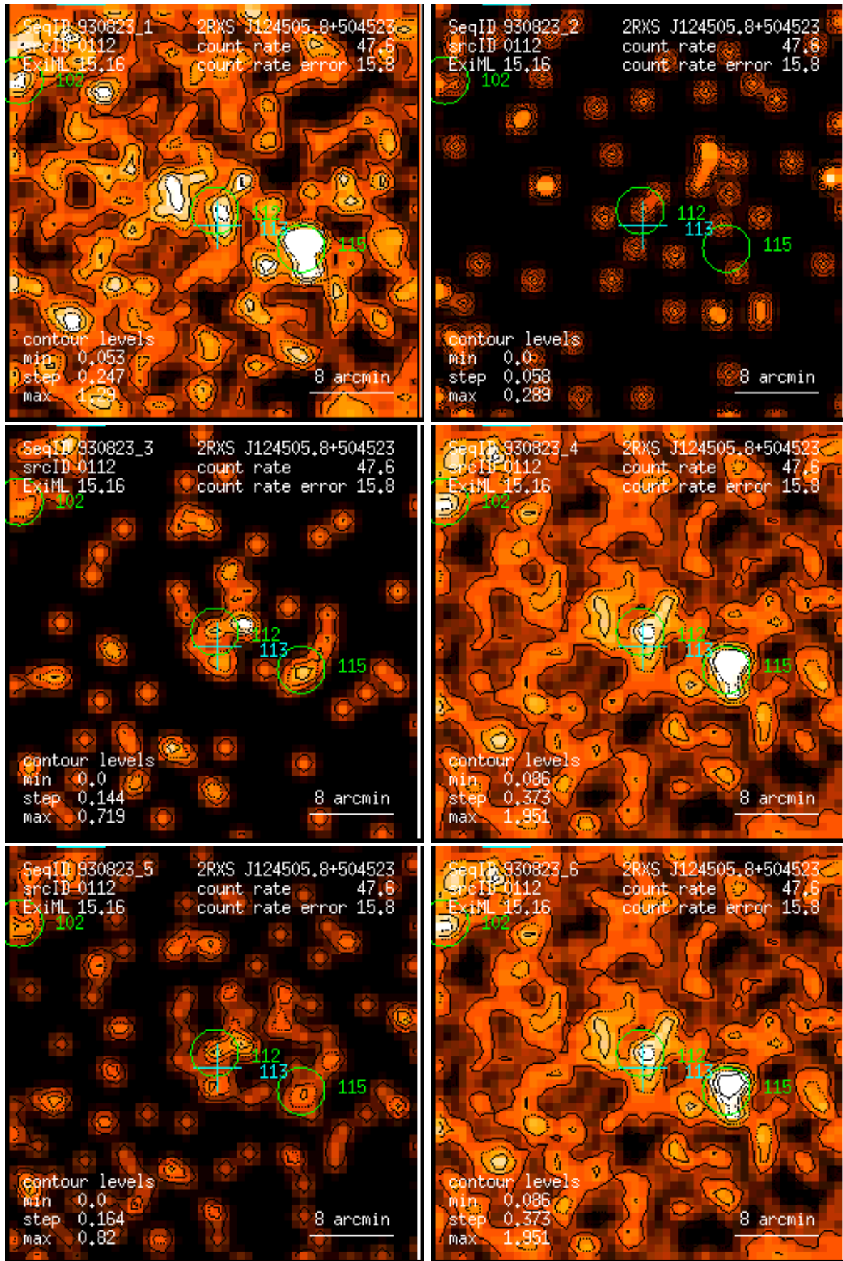
Figure 112: RASS 930823: detection 0112: band rate images, Gaussian filter: (1) PSPC channels 11 – 41, (2) 52 – 90, (3) 91 – 201, (4) 11 – 235, (5) 52 – 201, (6) 11 – 201. Broad band rates in counts/ks. Band rate contour levels in counts/ks/arcmin 2 .
