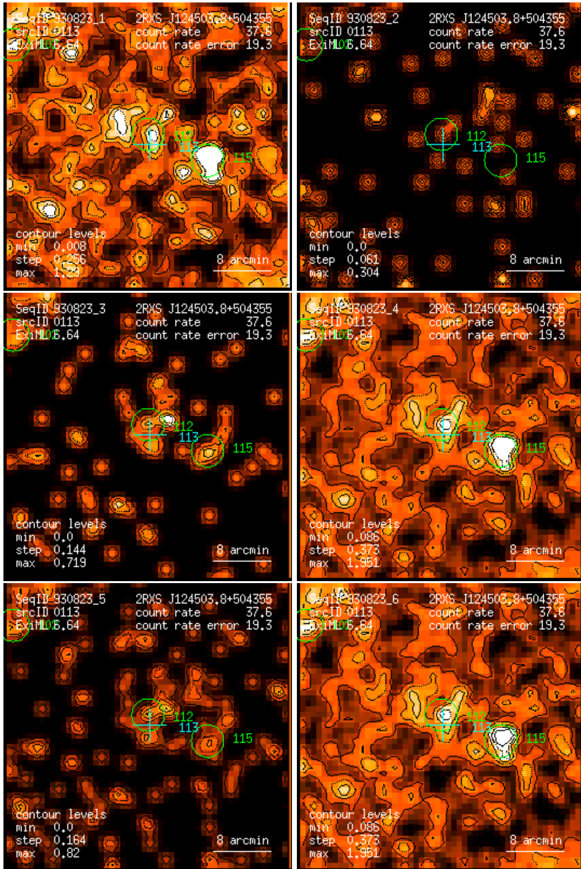
Figure 113: RASS 930823: detection 0113: band rate images, Gaussian filter: (1) PSPC channels 11 – 41, (2) 52 – 90, (3) 91 – 201, (4) 11 – 235, (5) 52 – 201, (6) 11 – 201. Broad band rates in counts/ks. Band rate contour levels in counts/ks/arcmin 2 .
