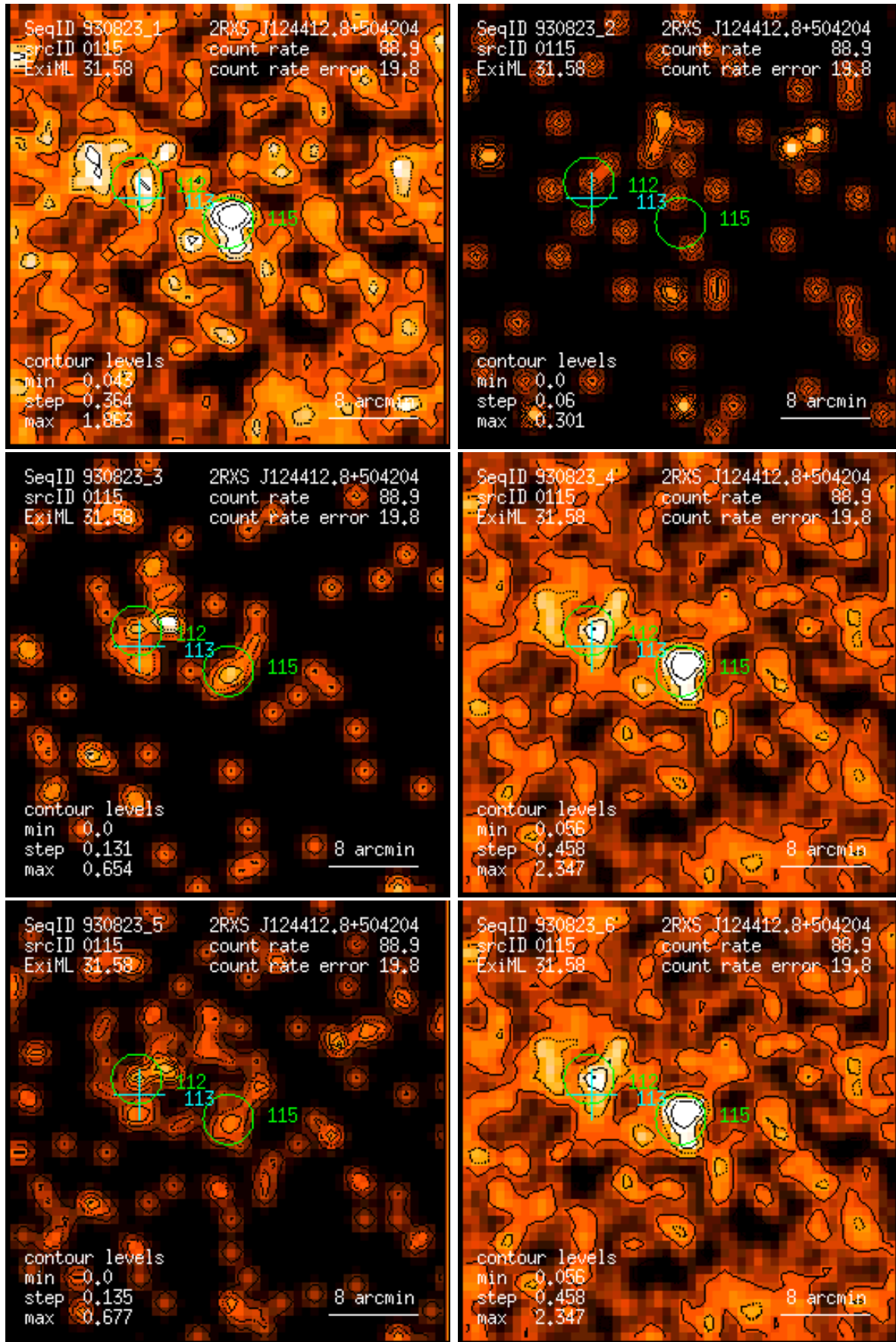
Figure 115: RASS 930823: detection 0115: band rate images, Gaussian filter: (1) PSPC channels 11 – 41, (2) 52 – 90, (3) 91 – 201, (4) 11 – 235, (5) 52 – 201, (6) 11 – 201. Broad band rates in counts/ks. Band rate contour levels in counts/ks/arcmin 2 .
