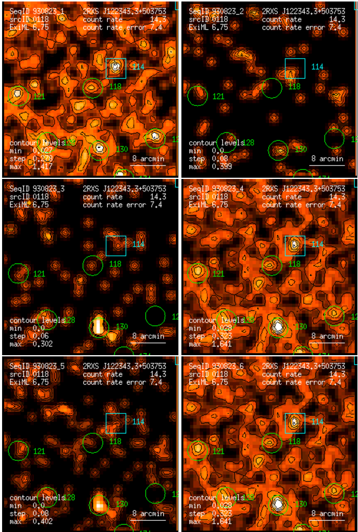
Figure 118: RASS 930823: detection 0118: band rate images, Gaussian filter: (1) PSPC channels 11 – 41, (2) 52 – 90, (3) 91 – 201, (4) 11 – 235, (5) 52 – 201, (6) 11 – 201. Broad band rates in counts/ks. Band rate contour levels in counts/ks/arcmin 2 .
