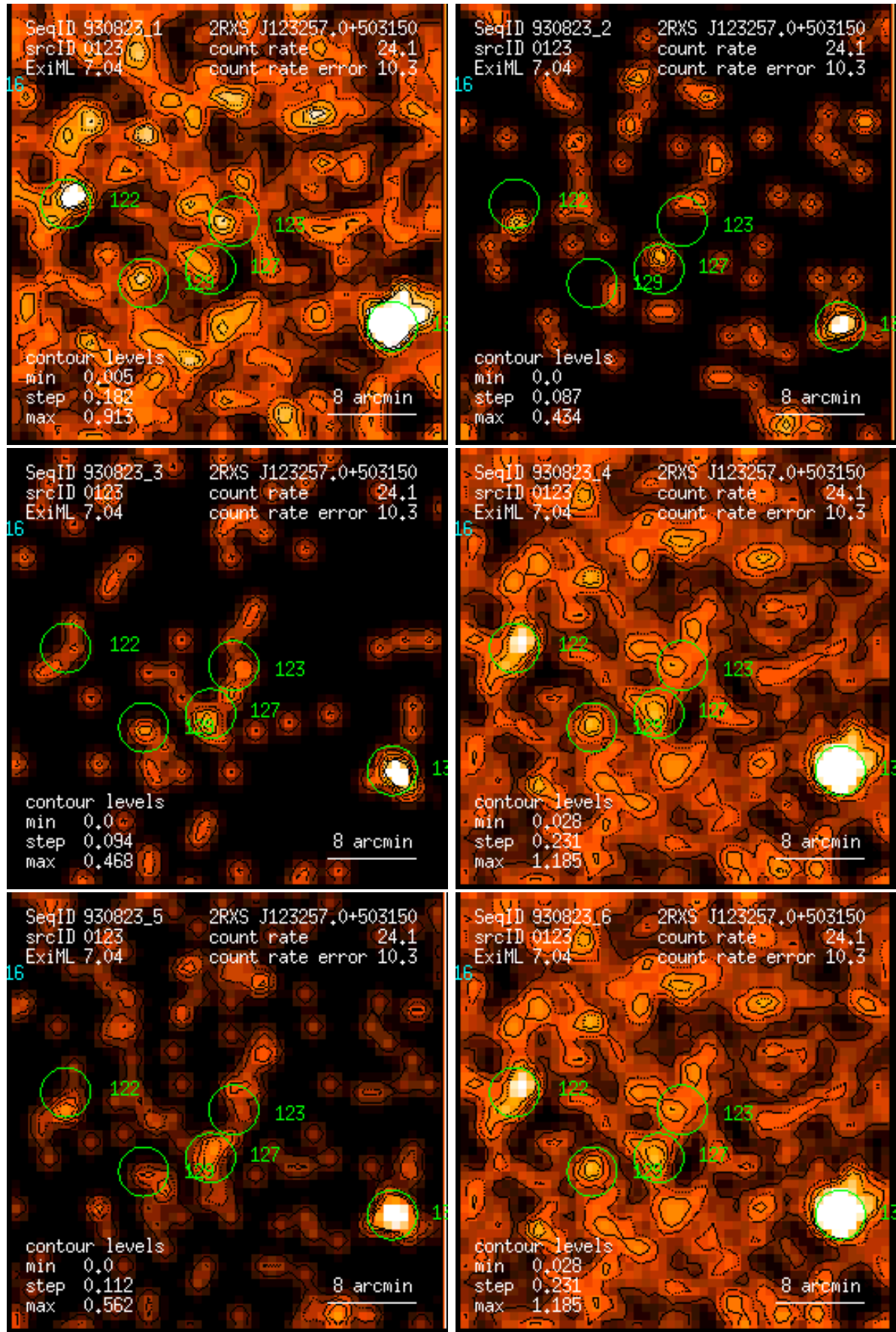
Figure 123: RASS 930823: detection 0123: band rate images, Gaussian filter: (1) PSPC channels 11 – 41, (2) 52 – 90, (3) 91 – 201, (4) 11 – 235, (5) 52 – 201, (6) 11 – 201. Broad band rates in counts/ks. Band rate contour levels in counts/ks/arcmin 2 .
