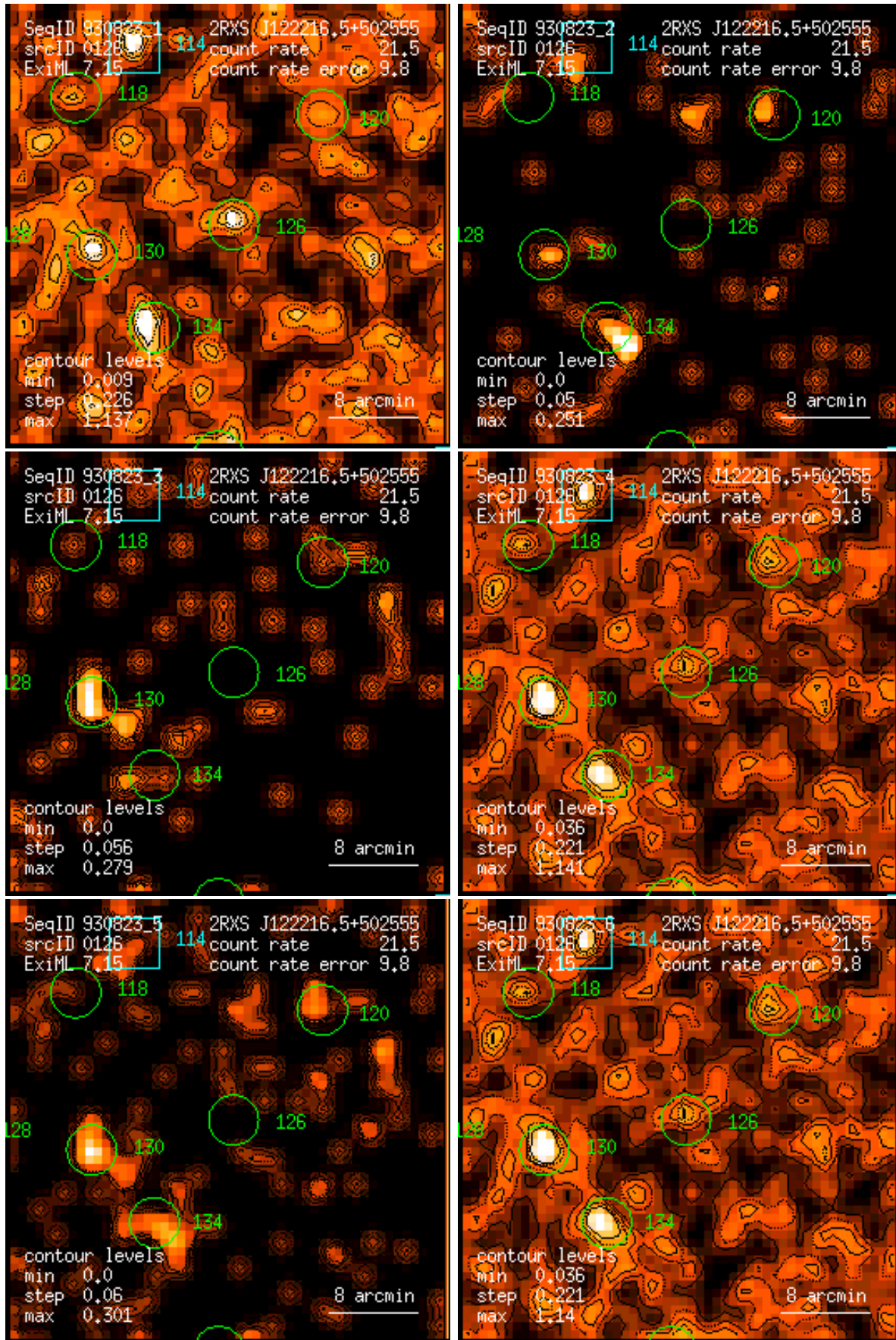
Figure 126: RASS 930823: detection 0126: band rate images, Gaussian filter: (1) PSPC channels 11 – 41, (2) 52 – 90, (3) 91 – 201, (4) 11 – 235, (5) 52 – 201, (6) 11 – 201. Broad band rates in counts/ks. Band rate contour levels in counts/ks/arcmin 2 .
