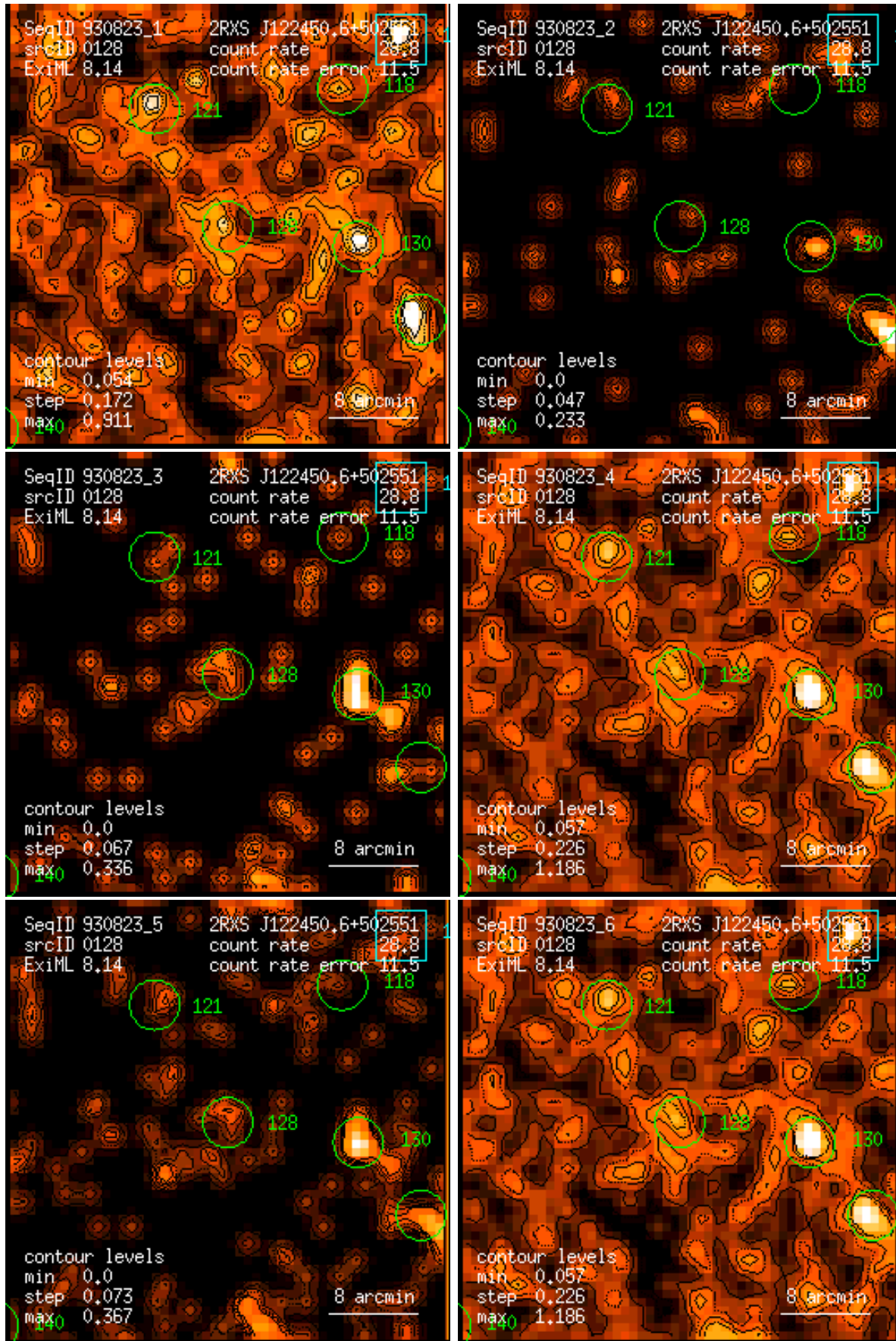
Figure 128: RASS 930823: detection 0128: band rate images, Gaussian filter: (1) PSPC channels 11 – 41, (2) 52 – 90, (3) 91 – 201, (4) 11 – 235, (5) 52 – 201, (6) 11 – 201. Broad band rates in counts/ks. Band rate contour levels in counts/ks/arcmin 2 .
