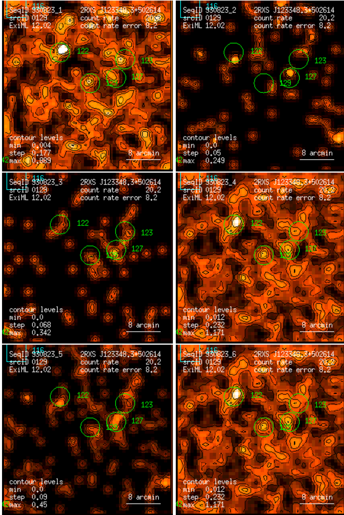
Figure 129: RASS 930823: detection 0129: band rate images, Gaussian filter: (1) PSPC channels 11 – 41, (2) 52 – 90, (3) 91 – 201, (4) 11 – 235, (5) 52 – 201, (6) 11 – 201. Broad band rates in counts/ks. Band rate contour levels in counts/ks/arcmin 2 .
