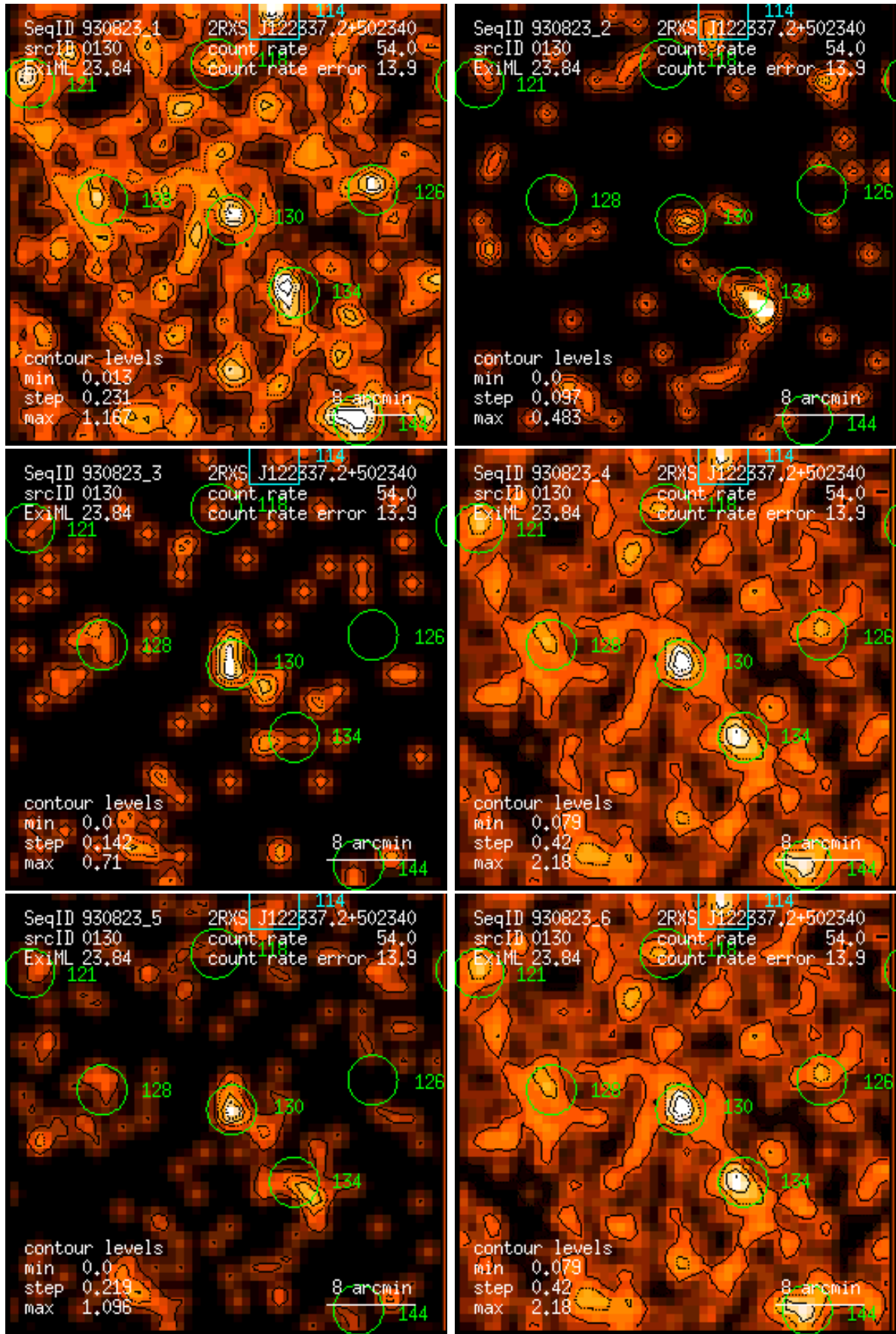
Figure 130: RASS 930823: detection 0130: band rate images, Gaussian filter: (1) PSPC channels 11 – 41, (2) 52 – 90, (3) 91 – 201, (4) 11 – 235, (5) 52 – 201, (6) 11 – 201. Broad band rates in counts/ks. Band rate contour levels in counts/ks/arcmin 2 .
