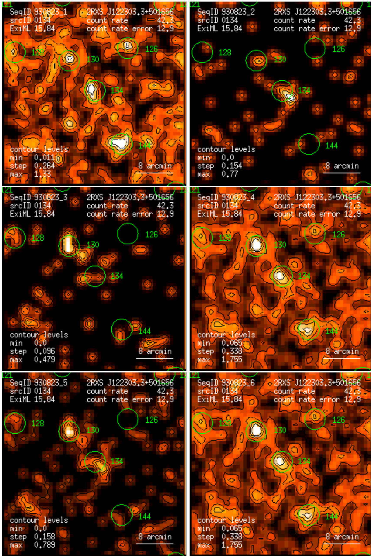
Figure 134: RASS 930823: detection 0134: band rate images, Gaussian filter: (1) PSPC channels 11 – 41, (2) 52 – 90, (3) 91 – 201, (4) 11 – 235, (5) 52 – 201, (6) 11 – 201. Broad band rates in counts/ks. Band rate contour levels in counts/ks/arcmin 2 .
