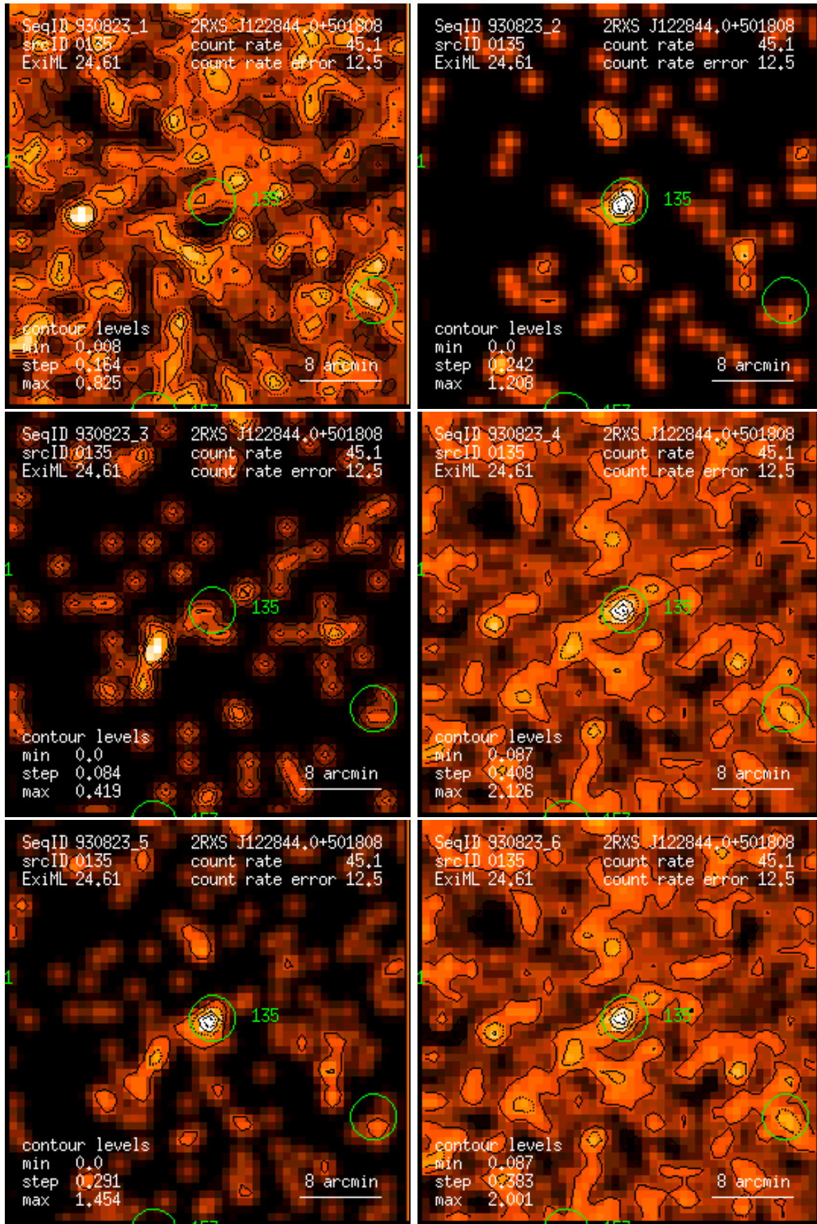
Figure 135: RASS 930823: detection 0135: band rate images, Gaussian filter: (1) PSPC channels 11 – 41, (2) 52 – 90, (3) 91 – 201, (4) 11 – 235, (5) 52 – 201, (6) 11 – 201. Broad band rates in counts/ks. Band rate contour levels in counts/ks/arcmin 2 .
