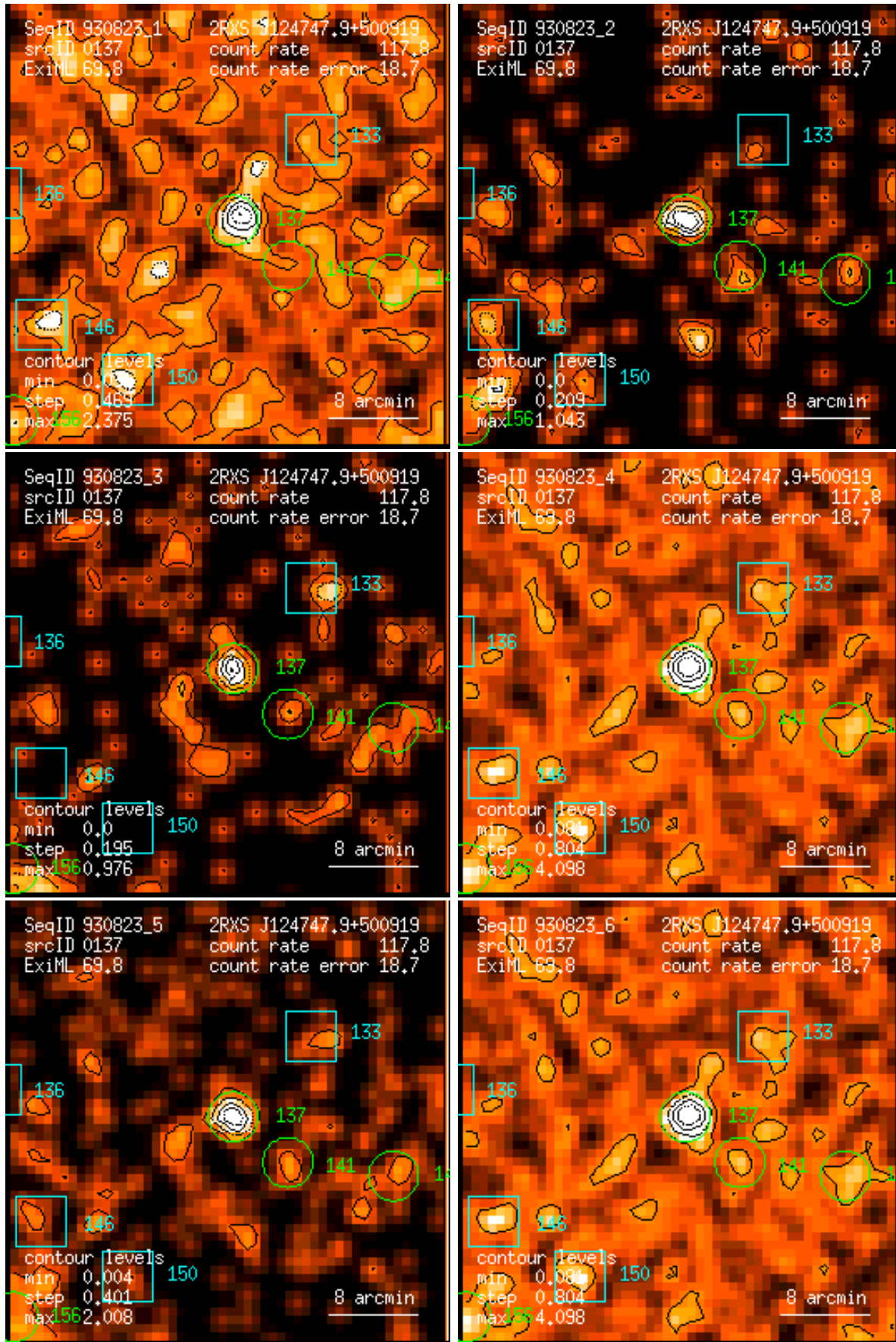
Figure 137: RASS 930823: detection 0137: band rate images, Gaussian filter: (1) PSPC channels 11 – 41, (2) 52 – 90, (3) 91 – 201, (4) 11 – 235, (5) 52 – 201, (6) 11 – 201. Broad band rates in counts/ks. Band rate contour levels in counts/ks/arcmin 2 .
