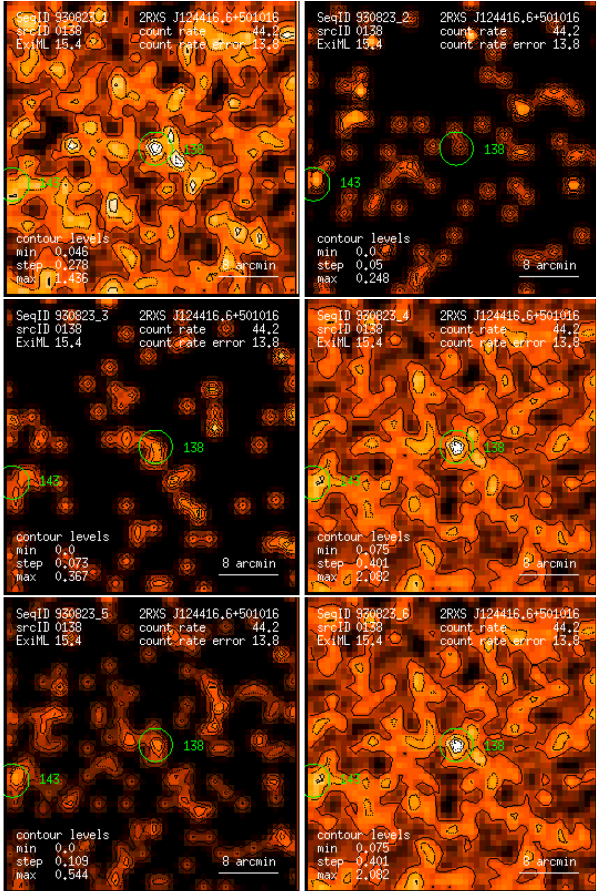
Figure 138: RASS 930823: detection 0138: band rate images, Gaussian filter: (1) PSPC channels 11 – 41, (2) 52 – 90, (3) 91 – 201, (4) 11 – 235, (5) 52 – 201, (6) 11 – 201. Broad band rates in counts/ks. Band rate contour levels in counts/ks/arcmin 2 .
