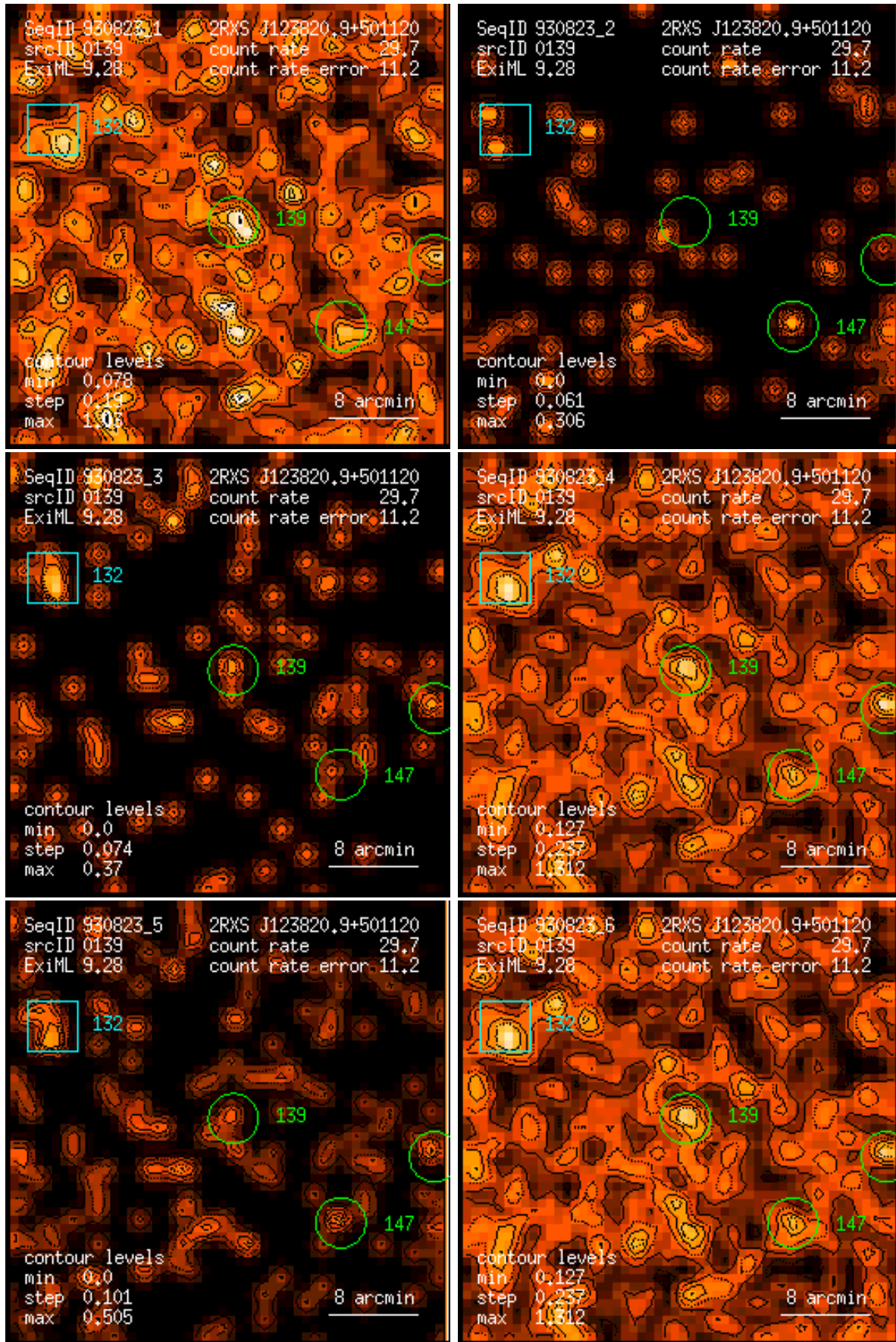
Figure 139: RASS 930823: detection 0139: band rate images, Gaussian filter: (1) PSPC channels 11 – 41, (2) 52 – 90, (3) 91 – 201, (4) 11 – 235, (5) 52 – 201, (6) 11 – 201. Broad band rates in counts/ks. Band rate contour levels in counts/ks/arcmin 2 .
