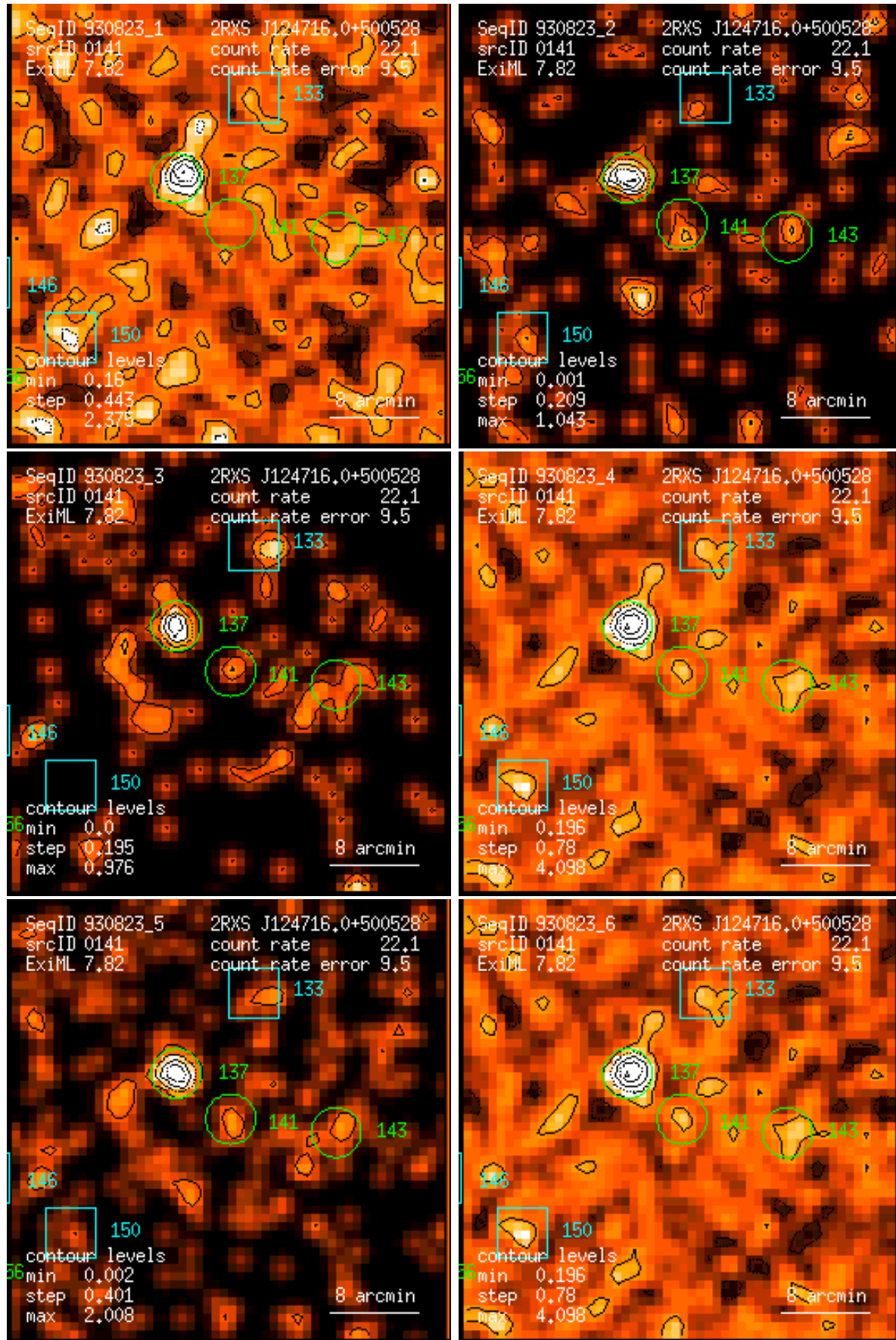
Figure 141: RASS 930823: detection 0141: band rate images, Gaussian filter: (1) PSPC channels 11 – 41, (2) 52 – 90, (3) 91 – 201, (4) 11 – 235, (5) 52 – 201, (6) 11 – 201. Broad band rates in counts/ks. Band rate contour levels in counts/ks/arcmin 2 .
