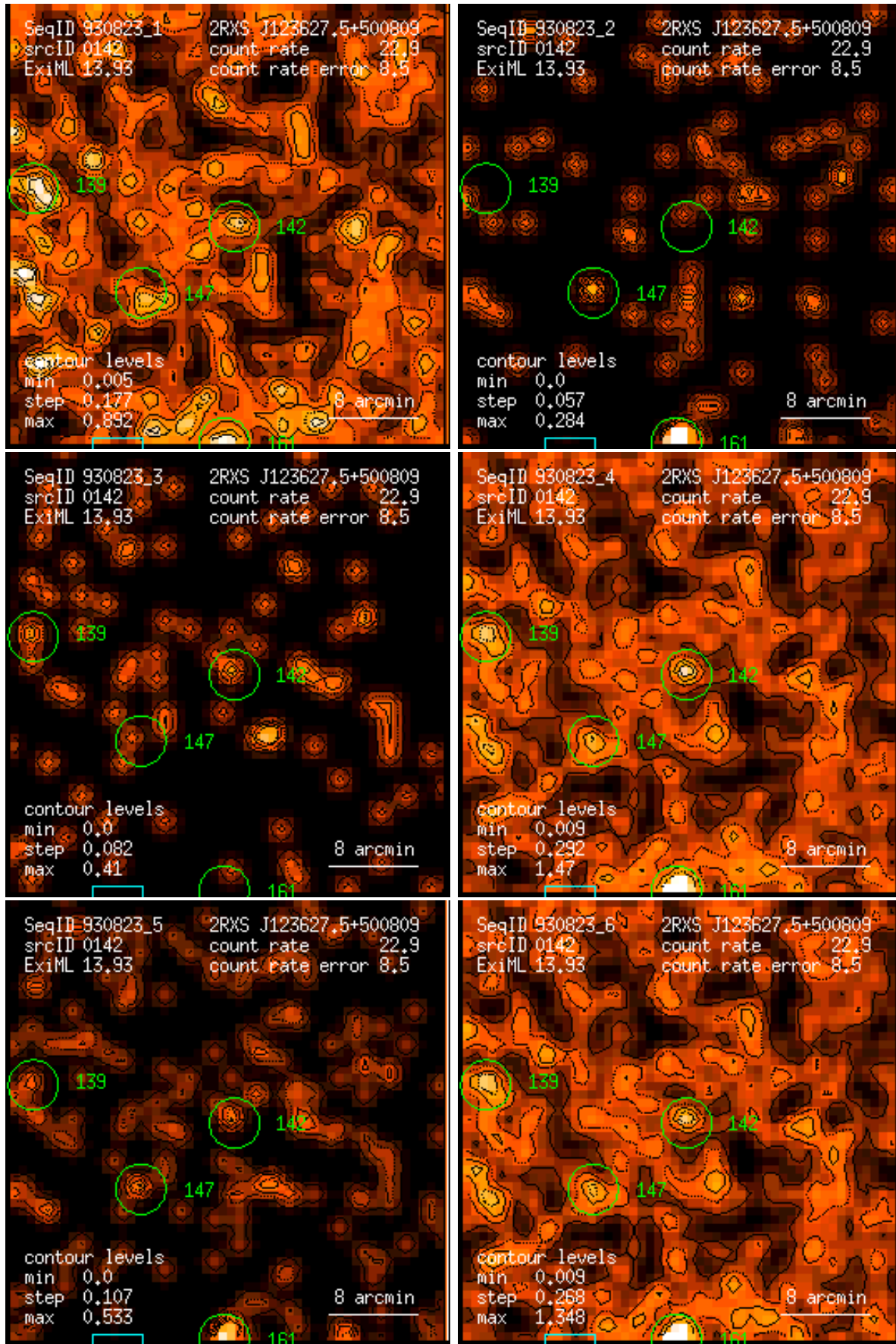
Figure 142: RASS 930823: detection 0142: band rate images, Gaussian filter: (1) PSPC channels 11 – 41, (2) 52 – 90, (3) 91 – 201, (4) 11 – 235, (5) 52 – 201, (6) 11 – 201. Broad band rates in counts/ks. Band rate contour levels in counts/ks/arcmin 2 .
