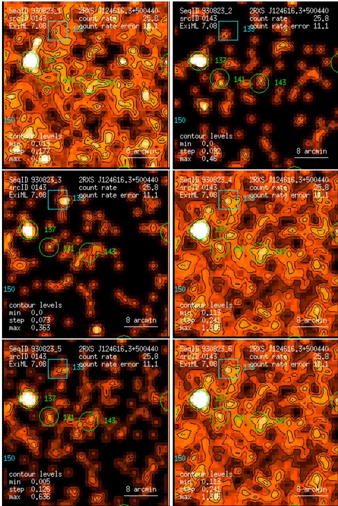
Figure 143: RASS 930823: detection 0143: band rate images, Gaussian filter: (1) PSPC channels 11 – 41, (2) 52 – 90, (3) 91 – 201, (4) 11 – 235, (5) 52 – 201, (6) 11 – 201. Broad band rates in counts/ks. Band rate contour levels in counts/ks/arcmin 2 .
