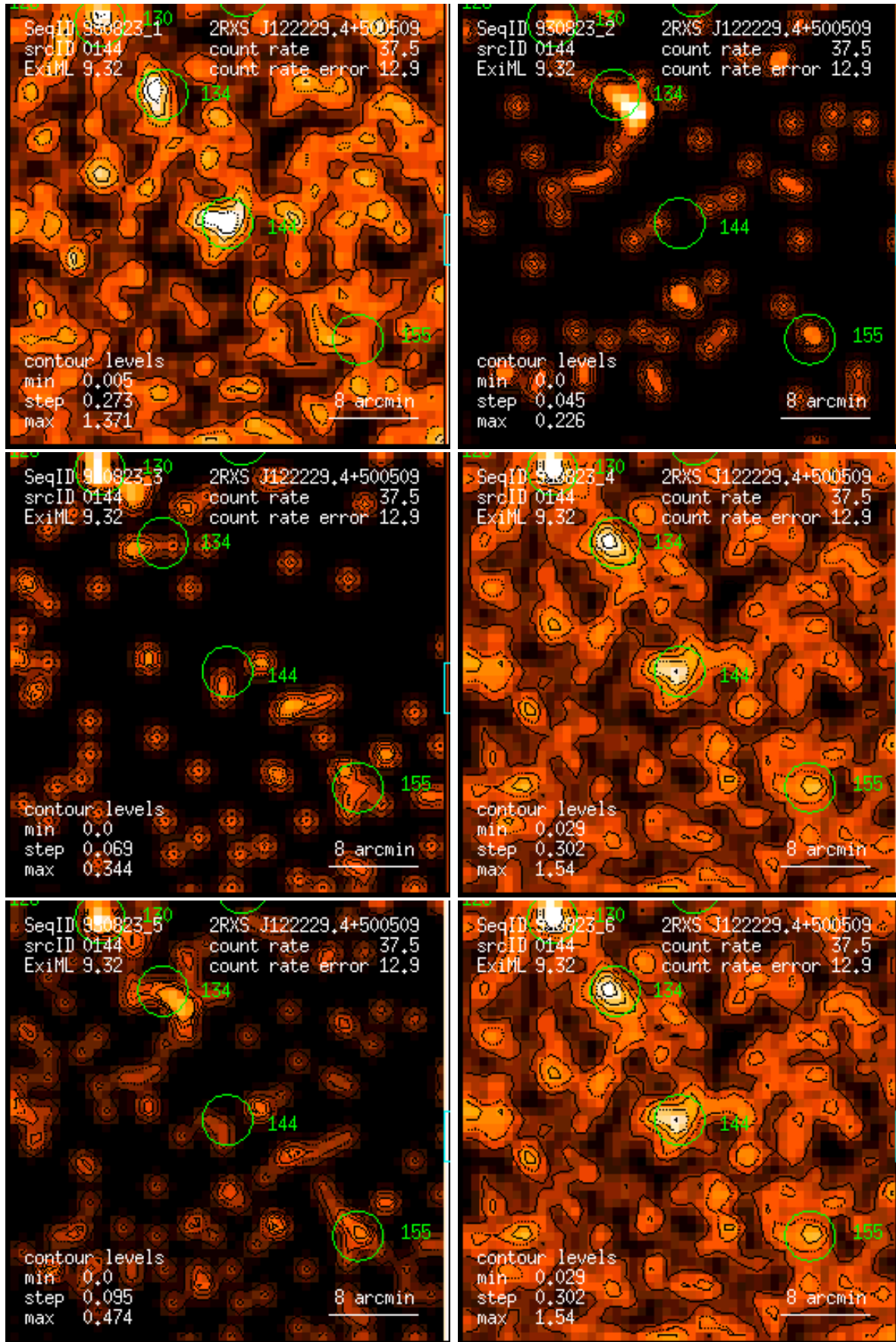
Figure 144: RASS 930823: detection 0144: band rate images, Gaussian filter: (1) PSPC channels 11 – 41, (2) 52 – 90, (3) 91 – 201, (4) 11 – 235, (5) 52 – 201, (6) 11 – 201. Broad band rates in counts/ks. Band rate contour levels in counts/ks/arcmin 2 .
