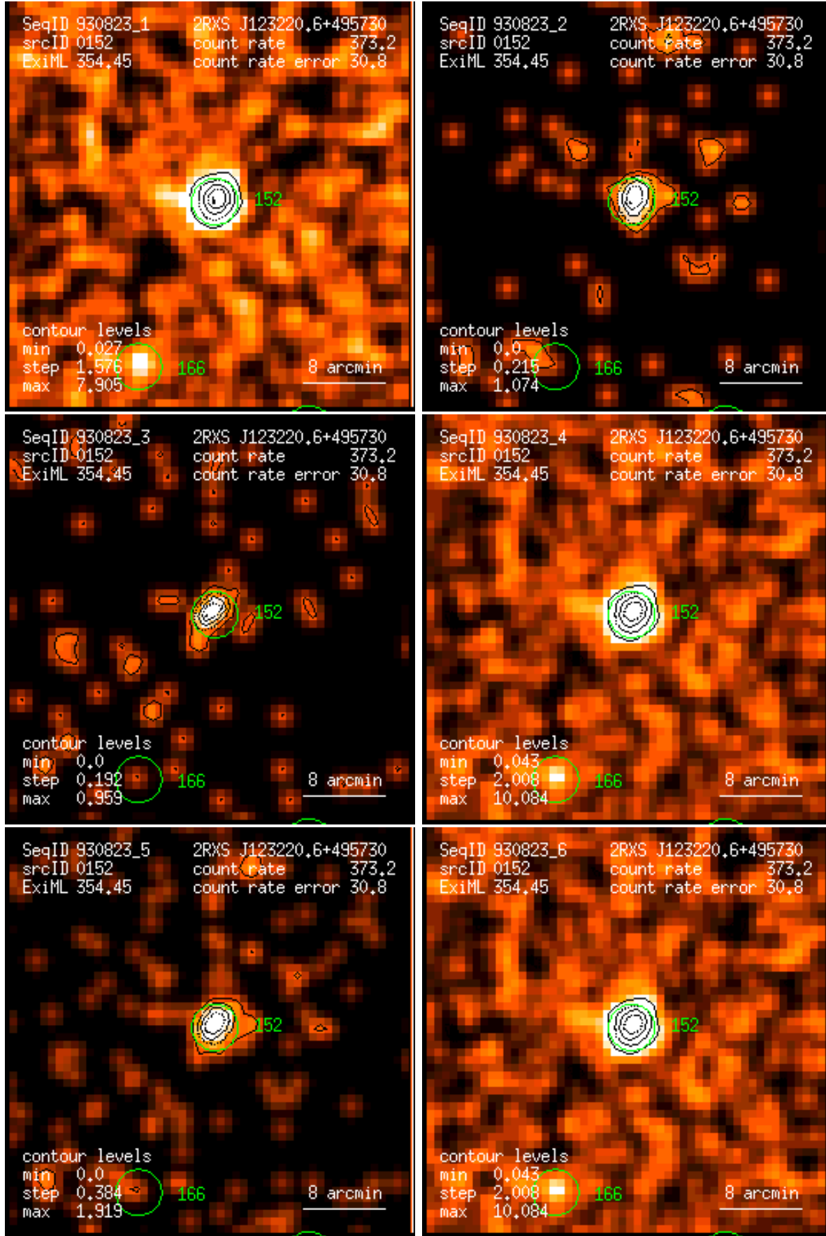
Figure 152: RASS 930823: detection 0152: band rate images, Gaussian filter: (1) PSPC channels 11 – 41, (2) 52 – 90, (3) 91 – 201, (4) 11 – 235, (5) 52 – 201, (6) 11 – 201. Broad band rates in counts/ks. Band rate contour levels in counts/ks/arcmin 2 .
