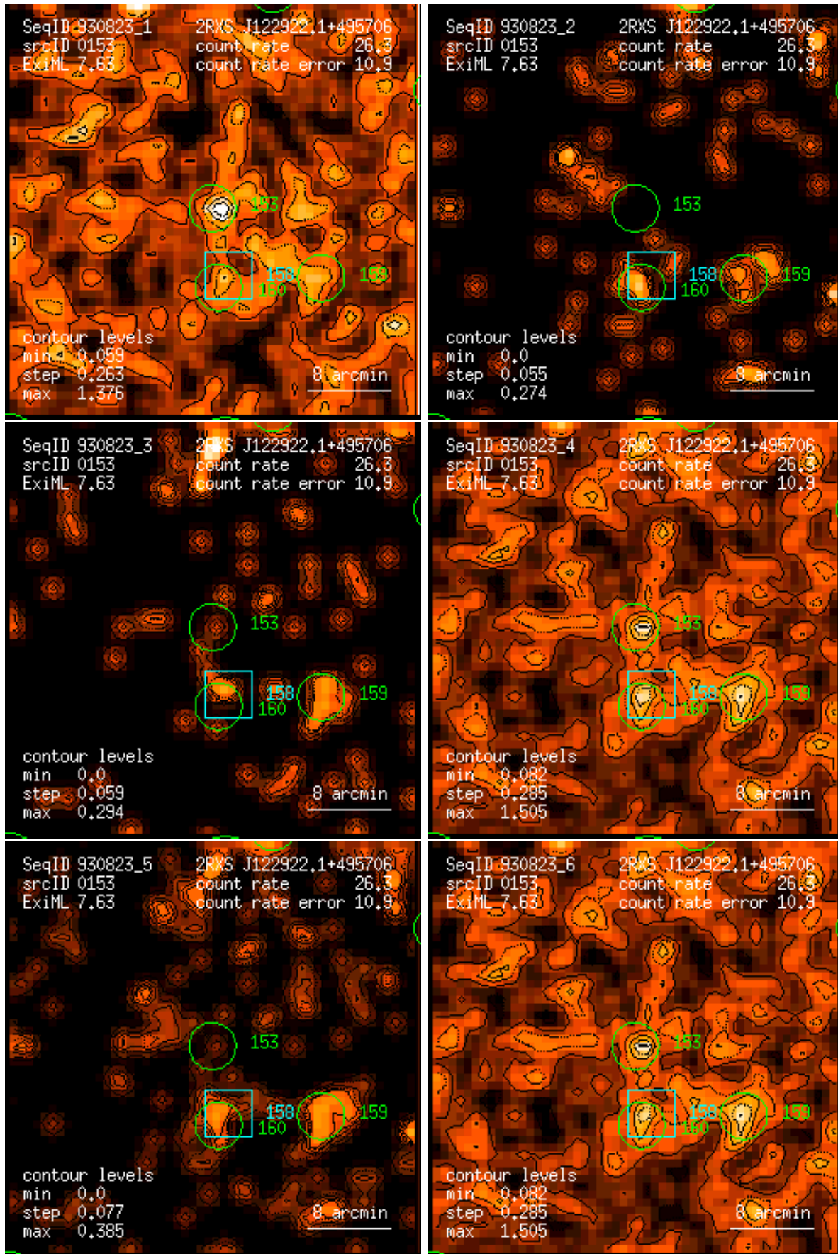
Figure 153: RASS 930823: detection 0153: band rate images, Gaussian filter: (1) PSPC channels 11 – 41, (2) 52 – 90, (3) 91 – 201, (4) 11 – 235, (5) 52 – 201, (6) 11 – 201. Broad band rates in counts/ks. Band rate contour levels in counts/ks/arcmin 2 .
