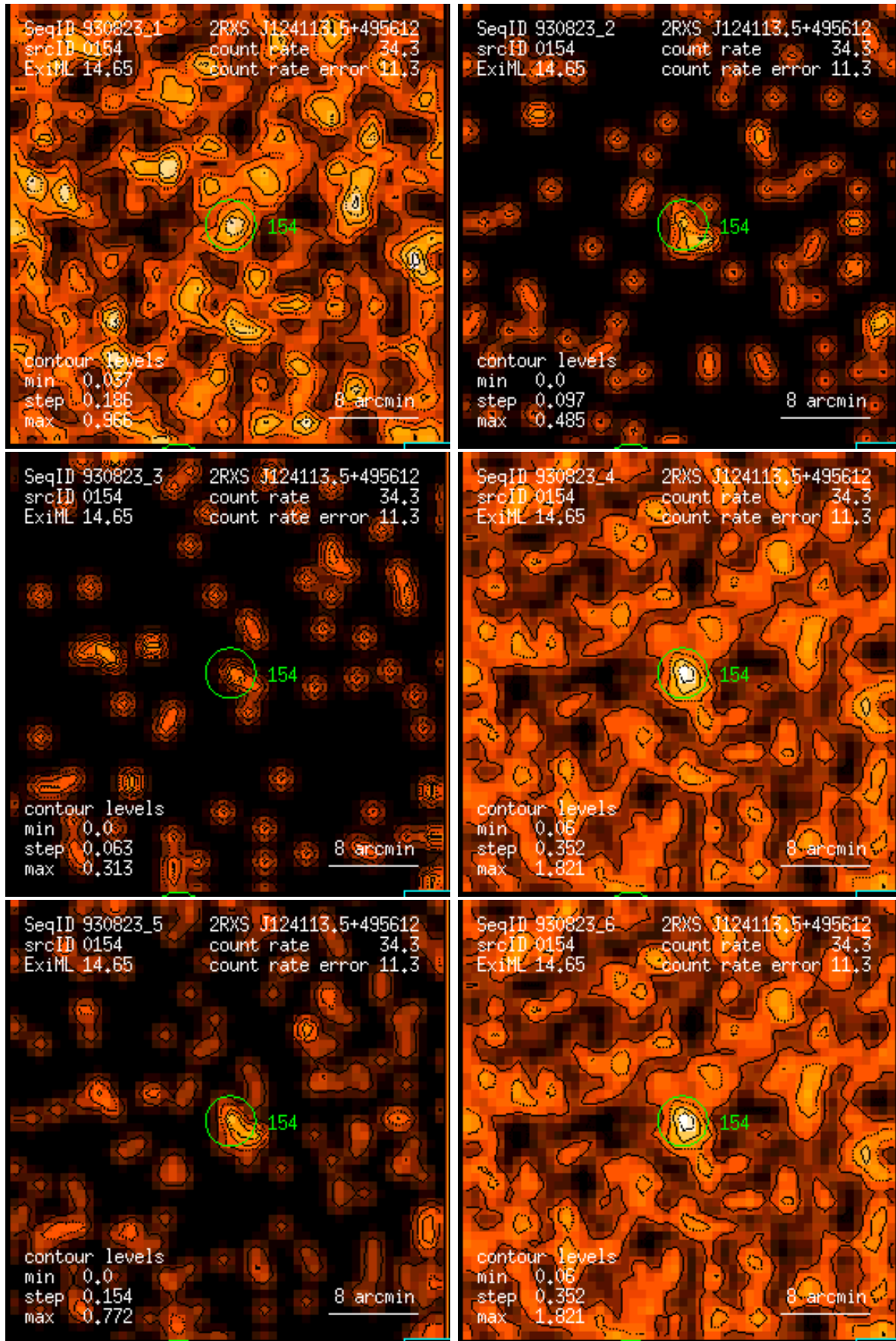
Figure 154: RASS 930823: detection 0154: band rate images, Gaussian filter: (1) PSPC channels 11 – 41, (2) 52 – 90, (3) 91 – 201, (4) 11 – 235, (5) 52 – 201, (6) 11 – 201. Broad band rates in counts/ks. Band rate contour levels in counts/ks/arcmin 2 .
