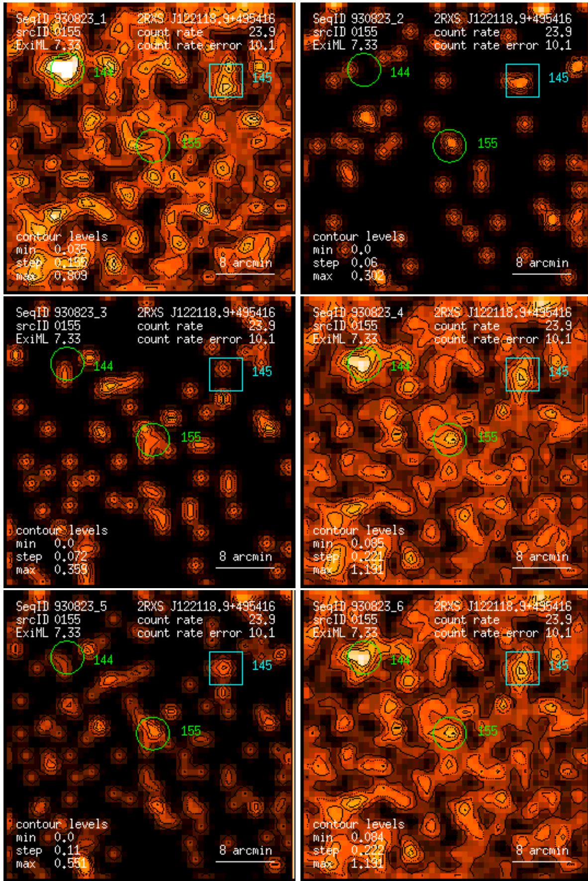
Figure 155: RASS 930823: detection 0155: band rate images, Gaussian filter: (1) PSPC channels 11 – 41, (2) 52 – 90, (3) 91 – 201, (4) 11 – 235, (5) 52 – 201, (6) 11 – 201. Broad band rates in counts/ks. Band rate contour levels in counts/ks/arcmin 2 .
