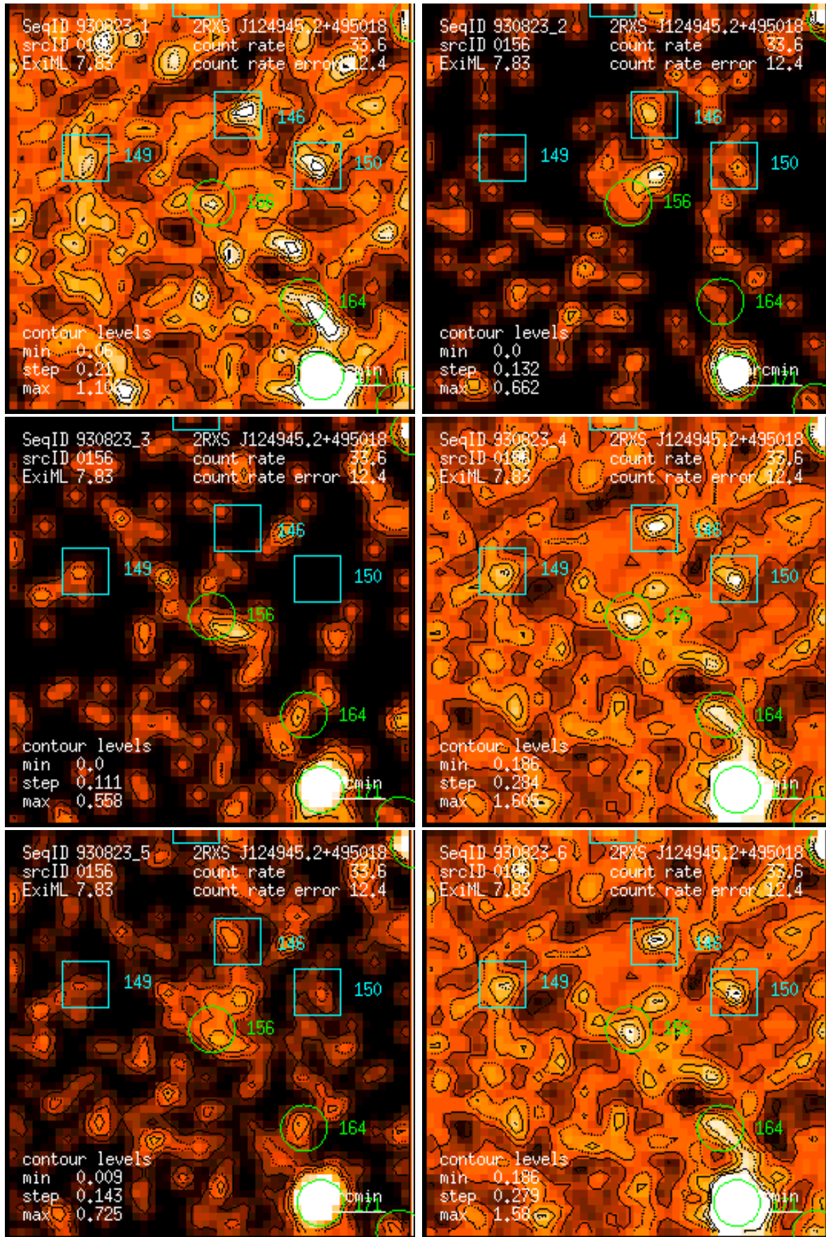
Figure 156: RASS 930823: detection 0156: band rate images, Gaussian filter: (1) PSPC channels 11 – 41, (2) 52 – 90, (3) 91 – 201, (4) 11 – 235, (5) 52 – 201, (6) 11 – 201. Broad band rates in counts/ks. Band rate contour levels in counts/ks/arcmin 2 .
