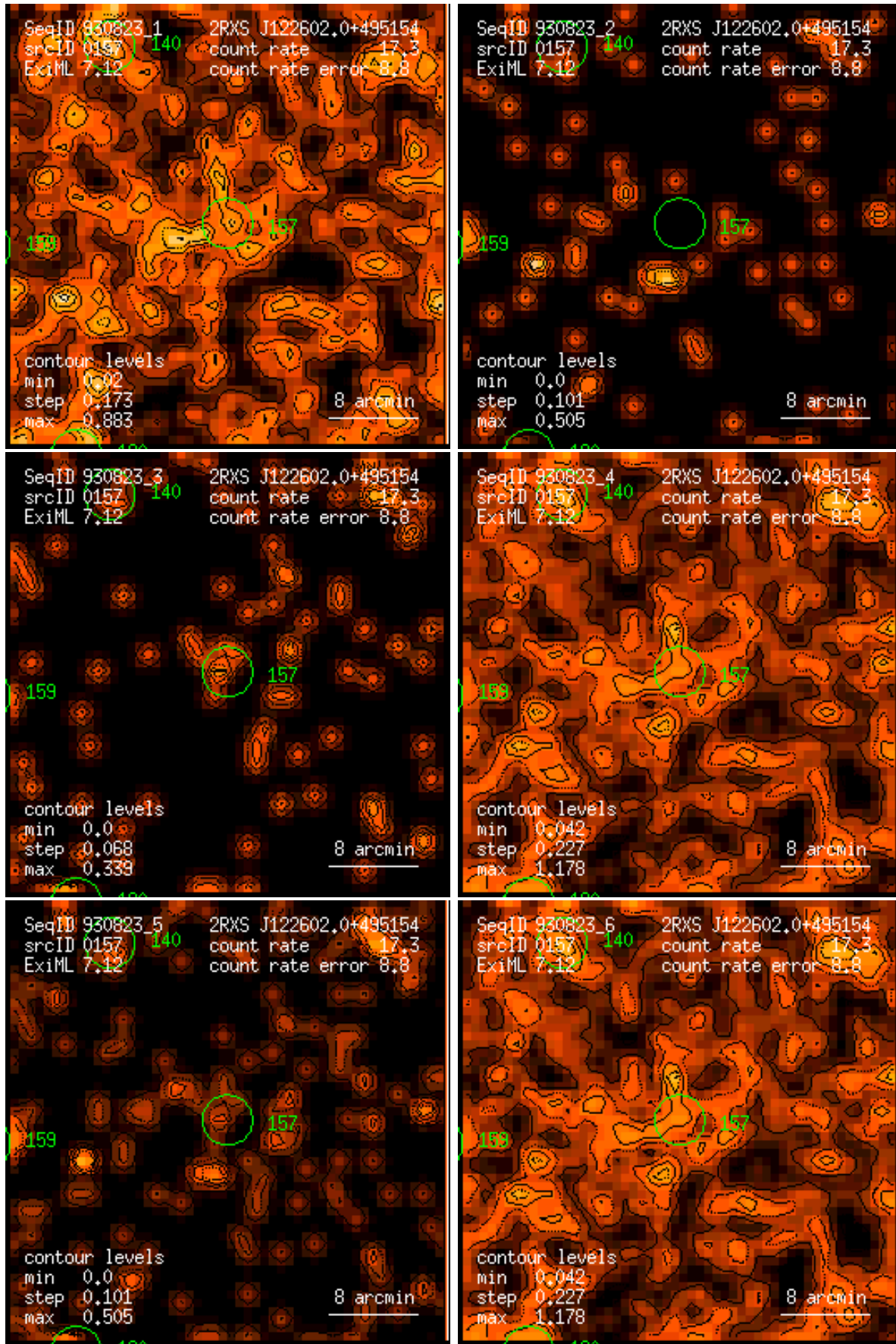
Figure 157: RASS 930823: detection 0157: band rate images, Gaussian filter: (1) PSPC channels 11 – 41, (2) 52 – 90, (3) 91 – 201, (4) 11 – 235, (5) 52 – 201, (6) 11 – 201. Broad band rates in counts/ks. Band rate contour levels in counts/ks/arcmin 2 .
