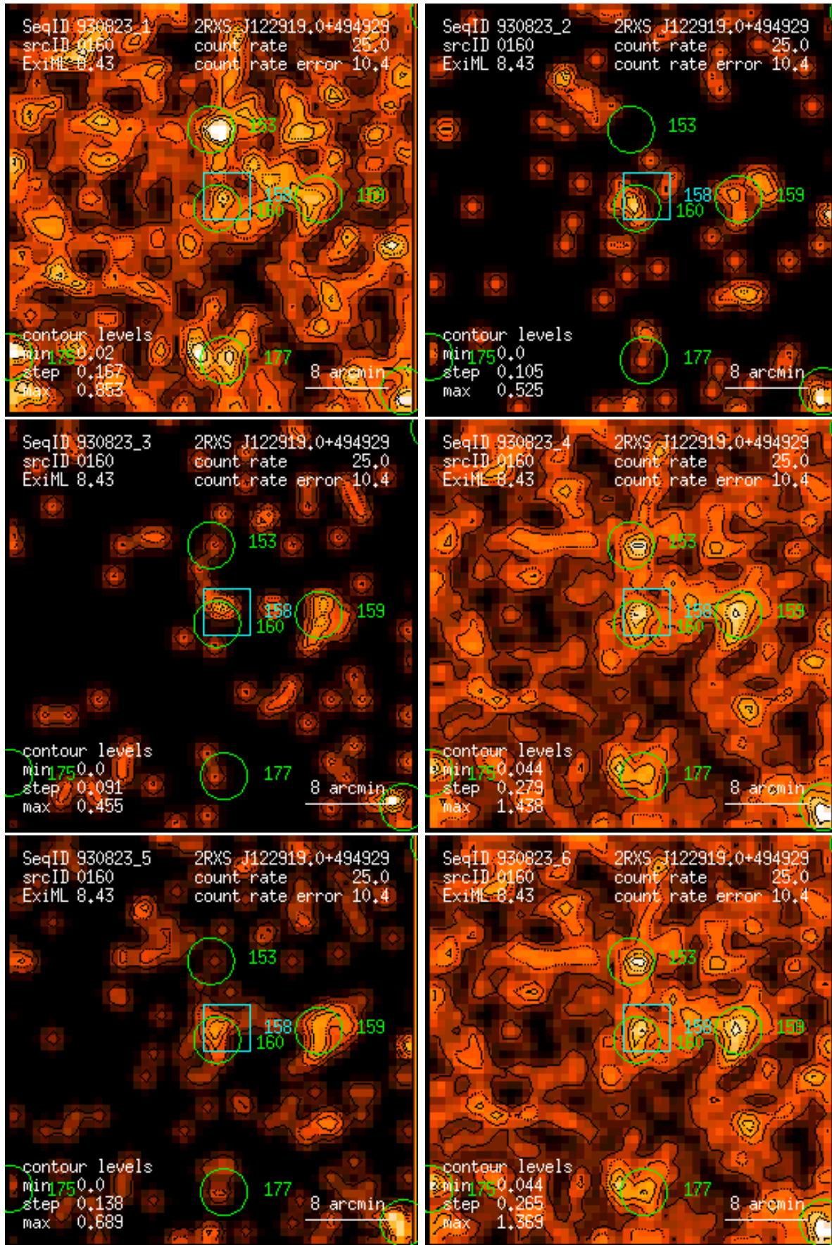
Figure 160: RASS 930823: detection 0160: band rate images, Gaussian filter: (1) PSPC channels 11 – 41, (2) 52 – 90, (3) 91 – 201, (4) 11 – 235, (5) 52 – 201, (6) 11 – 201. Broad band rates in counts/ks. Band rate contour levels in counts/ks/arcmin 2 .
