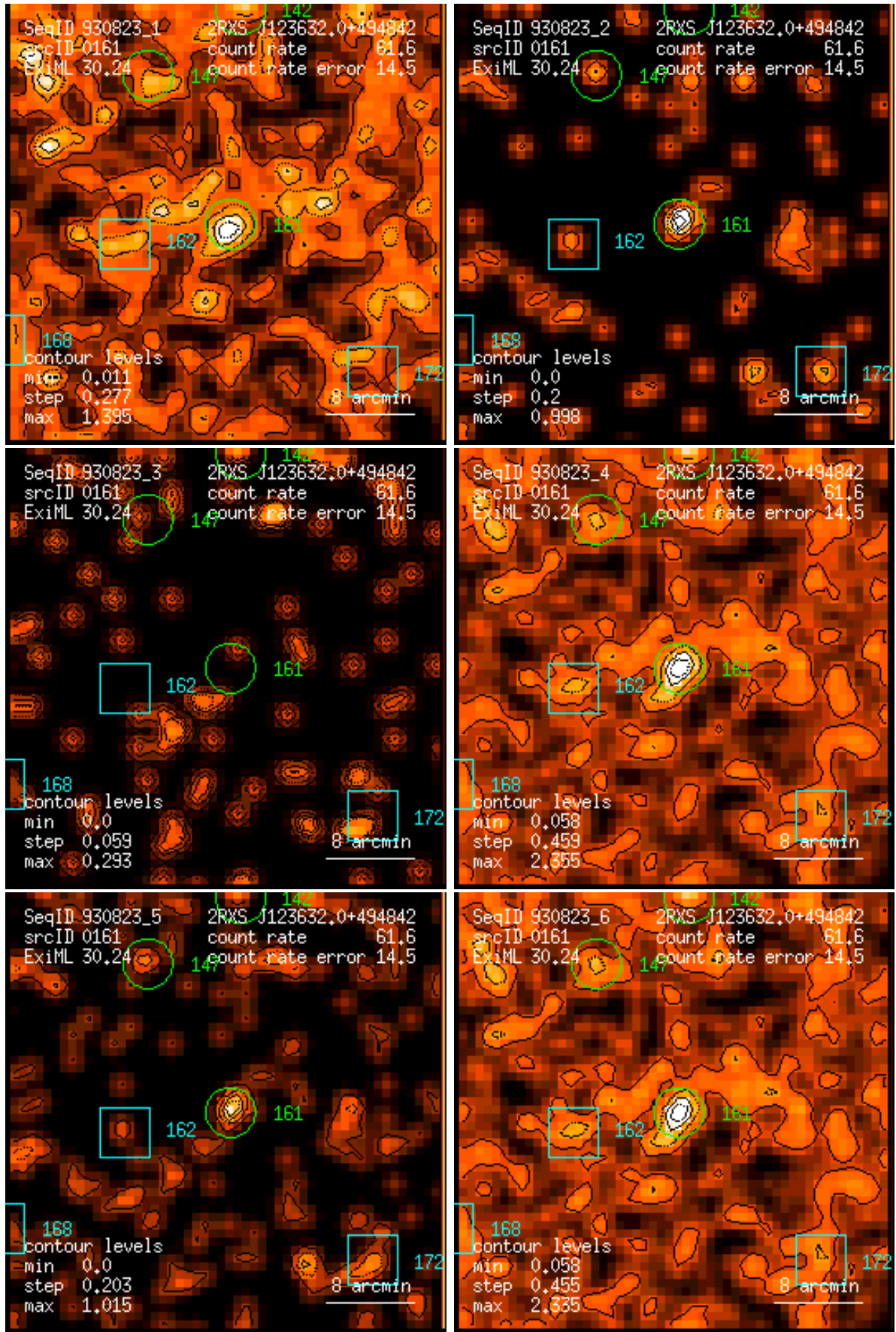
Figure 161: RASS 930823: detection 0161: band rate images, Gaussian filter: (1) PSPC channels 11 – 41, (2) 52 – 90, (3) 91 – 201, (4) 11 – 235, (5) 52 – 201, (6) 11 – 201. Broad band rates in counts/ks. Band rate contour levels in counts/ks/arcmin 2 .
