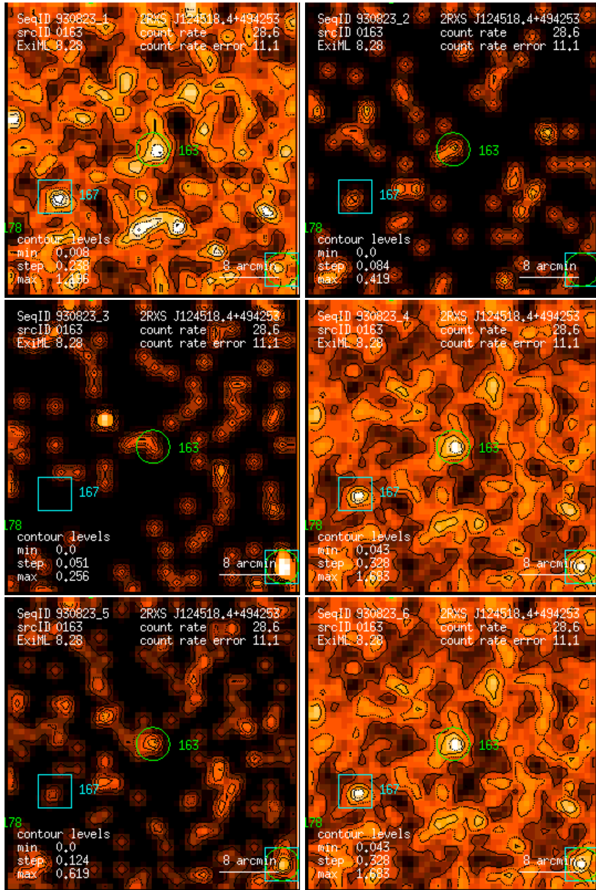
Figure 163: RASS 930823: detection 0163: band rate images, Gaussian filter: (1) PSPC channels 11 – 41, (2) 52 – 90, (3) 91 – 201, (4) 11 – 235, (5) 52 – 201, (6) 11 – 201. Broad band rates in counts/ks. Band rate contour levels in counts/ks/arcmin 2 .
