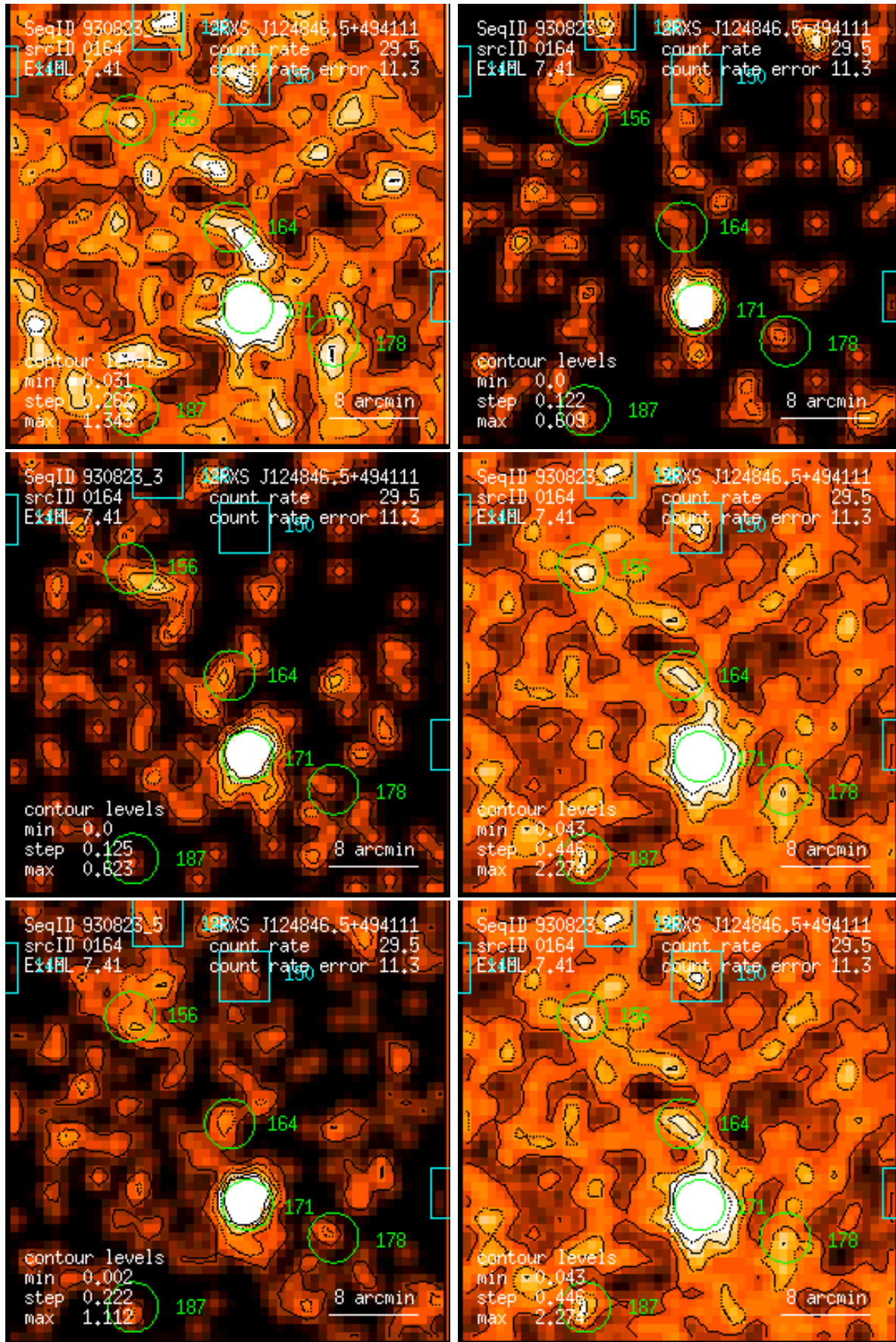
Figure 164: RASS 930823: detection 0164: band rate images, Gaussian filter: (1) PSPC channels 11 – 41, (2) 52 – 90, (3) 91 – 201, (4) 11 – 235, (5) 52 – 201, (6) 11 – 201. Broad band rates in counts/ks. Band rate contour levels in counts/ks/arcmin 2 .
