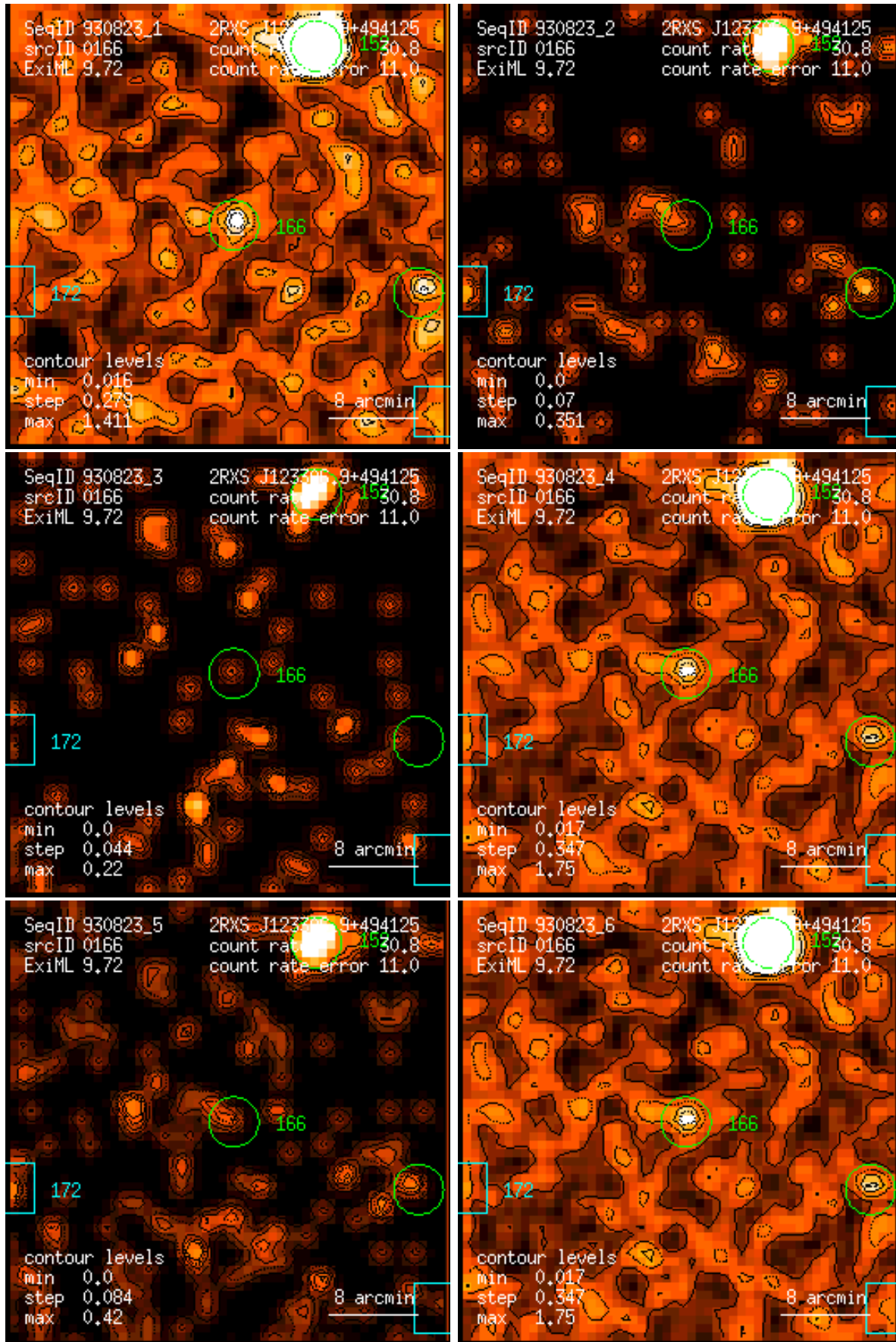
Figure 166: RASS 930823: detection 0166: band rate images, Gaussian filter: (1) PSPC channels 11 – 41, (2) 52 – 90, (3) 91 – 201, (4) 11 – 235, (5) 52 – 201, (6) 11 – 201. Broad band rates in counts/ks. Band rate contour levels in counts/ks/arcmin 2 .
