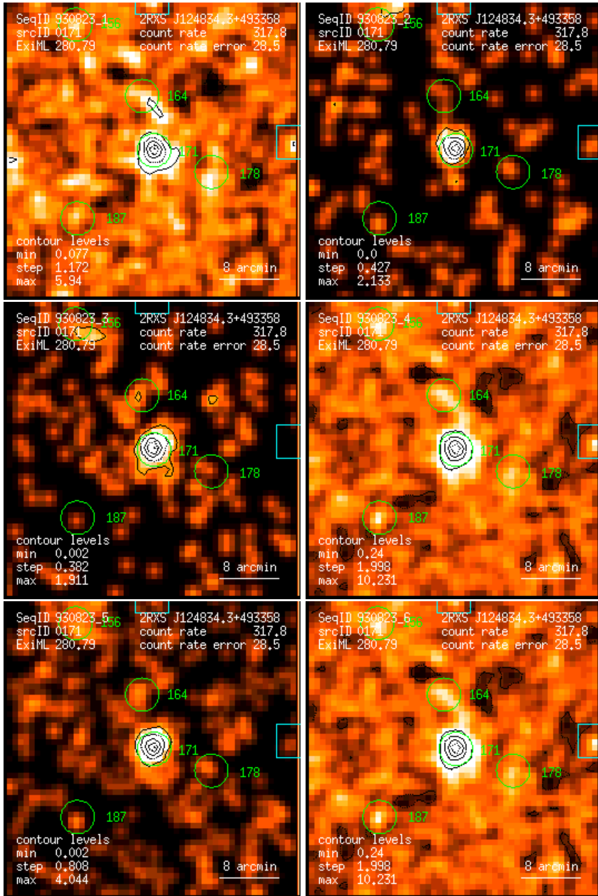
Figure 171: RASS 930823: detection 0171: band rate images, Gaussian filter: (1) PSPC channels 11 – 41, (2) 52 – 90, (3) 91 – 201, (4) 11 – 235, (5) 52 – 201, (6) 11 – 201. Broad band rates in counts/ks. Band rate contour levels in counts/ks/arcmin 2 .
