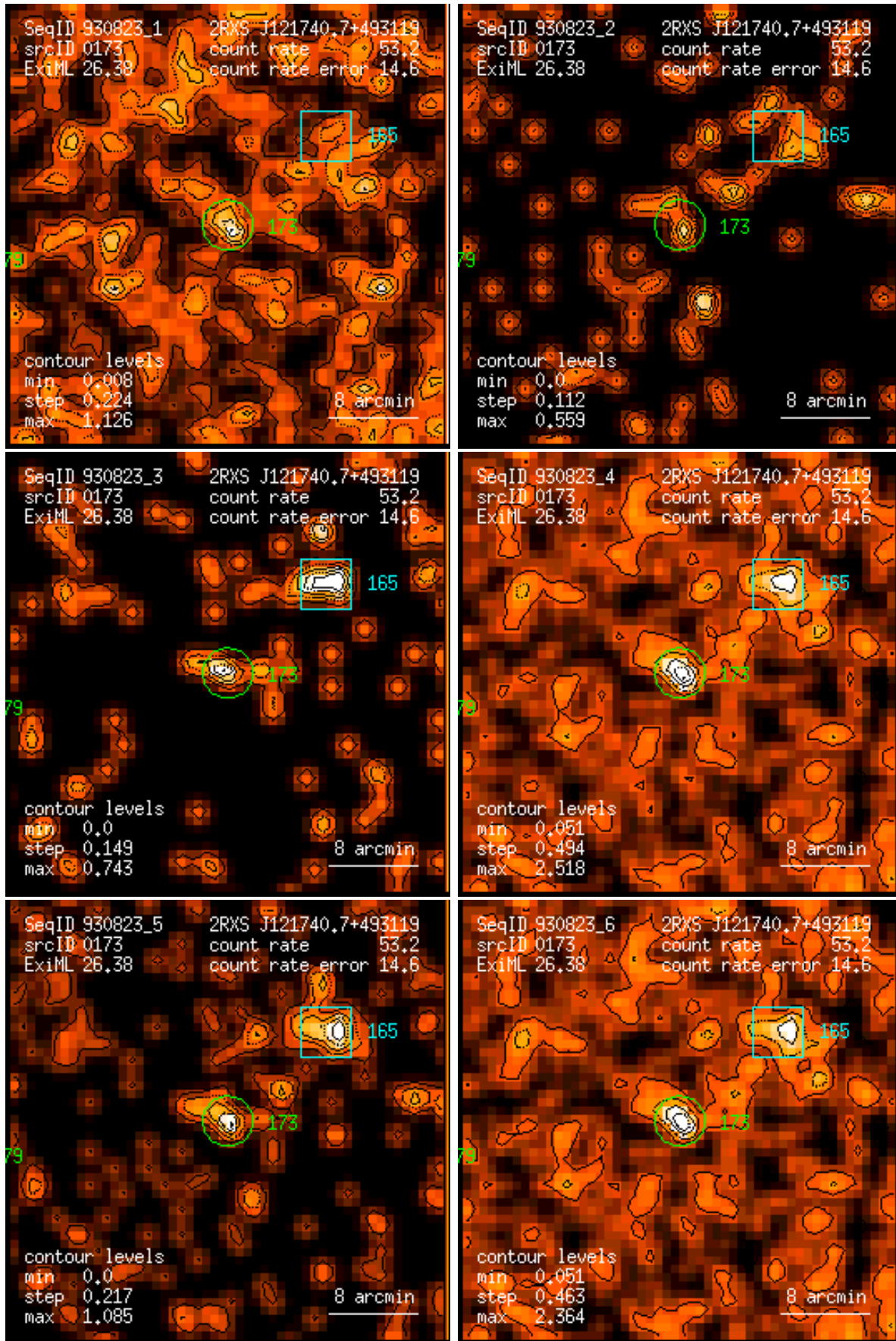
Figure 173: RASS 930823: detection 0173: band rate images, Gaussian filter: (1) PSPC channels 11 – 41, (2) 52 – 90, (3) 91 – 201, (4) 11 – 235, (5) 52 – 201, (6) 11 – 201. Broad band rates in counts/ks. Band rate contour levels in counts/ks/arcmin 2 .
