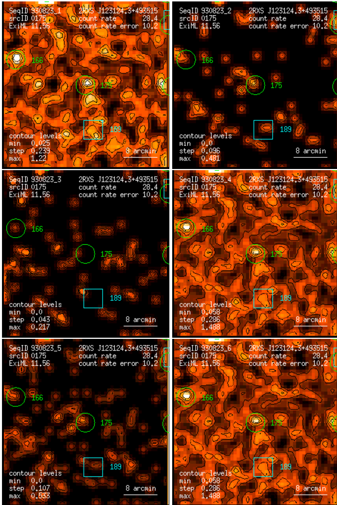
Figure 175: RASS 930823: detection 0175: band rate images, Gaussian filter: (1) PSPC channels 11 – 41, (2) 52 – 90, (3) 91 – 201, (4) 11 – 235, (5) 52 – 201, (6) 11 – 201. Broad band rates in counts/ks. Band rate contour levels in counts/ks/arcmin 2 .
