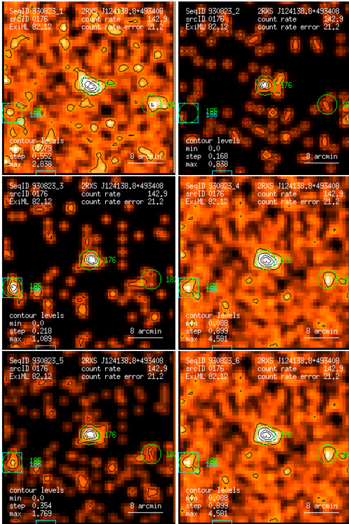
Figure 176: RASS 930823: detection 0176: band rate images, Gaussian filter: (1) PSPC channels 11 – 41, (2) 52 – 90, (3) 91 – 201, (4) 11 – 235, (5) 52 – 201, (6) 11 – 201. Broad band rates in counts/ks. Band rate contour levels in counts/ks/arcmin 2 .
