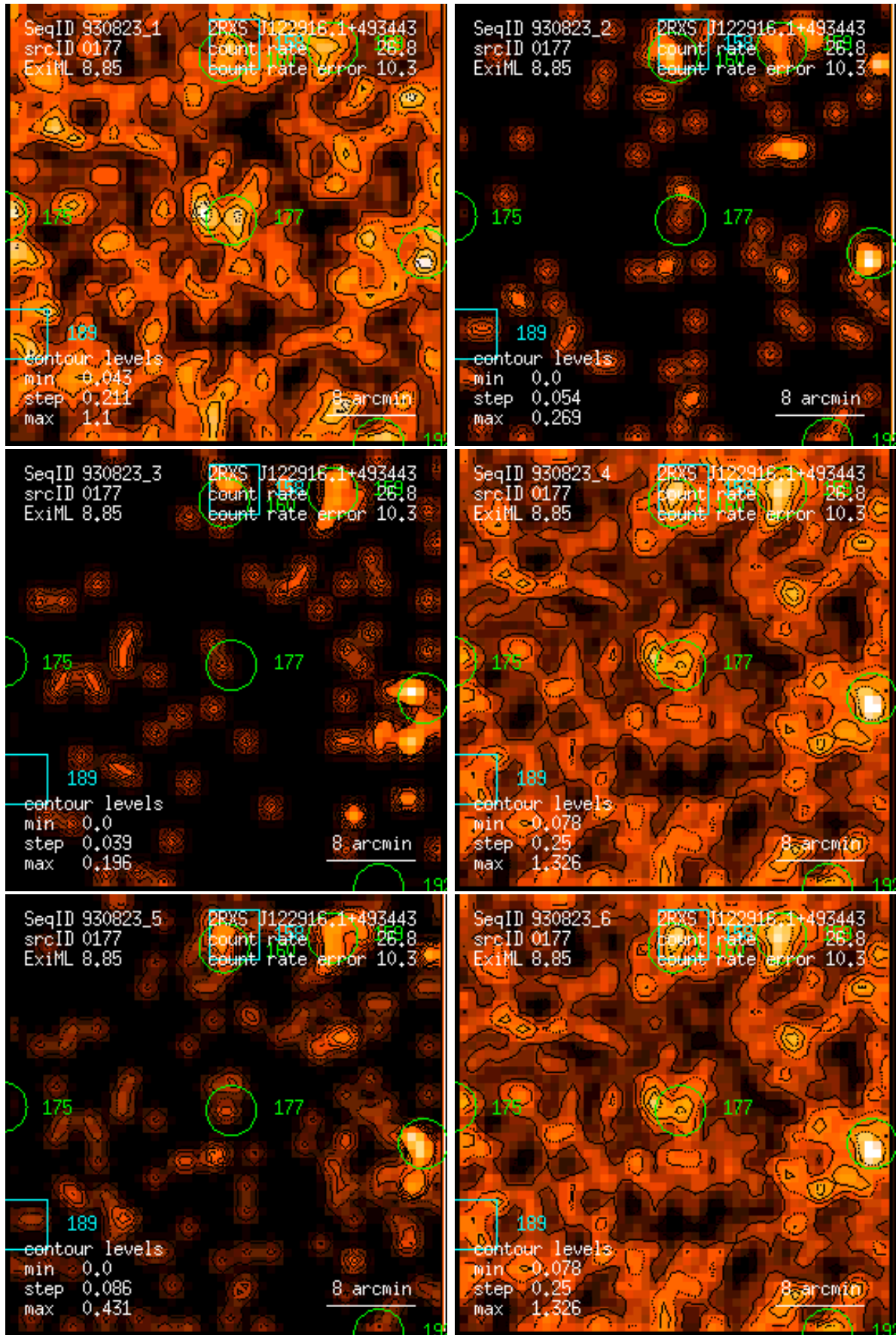
Figure 177: RASS 930823: detection 0177: band rate images, Gaussian filter: (1) PSPC channels 11 – 41, (2) 52 – 90, (3) 91 – 201, (4) 11 – 235, (5) 52 – 201, (6) 11 – 201. Broad band rates in counts/ks. Band rate contour levels in counts/ks/arcmin 2 .
